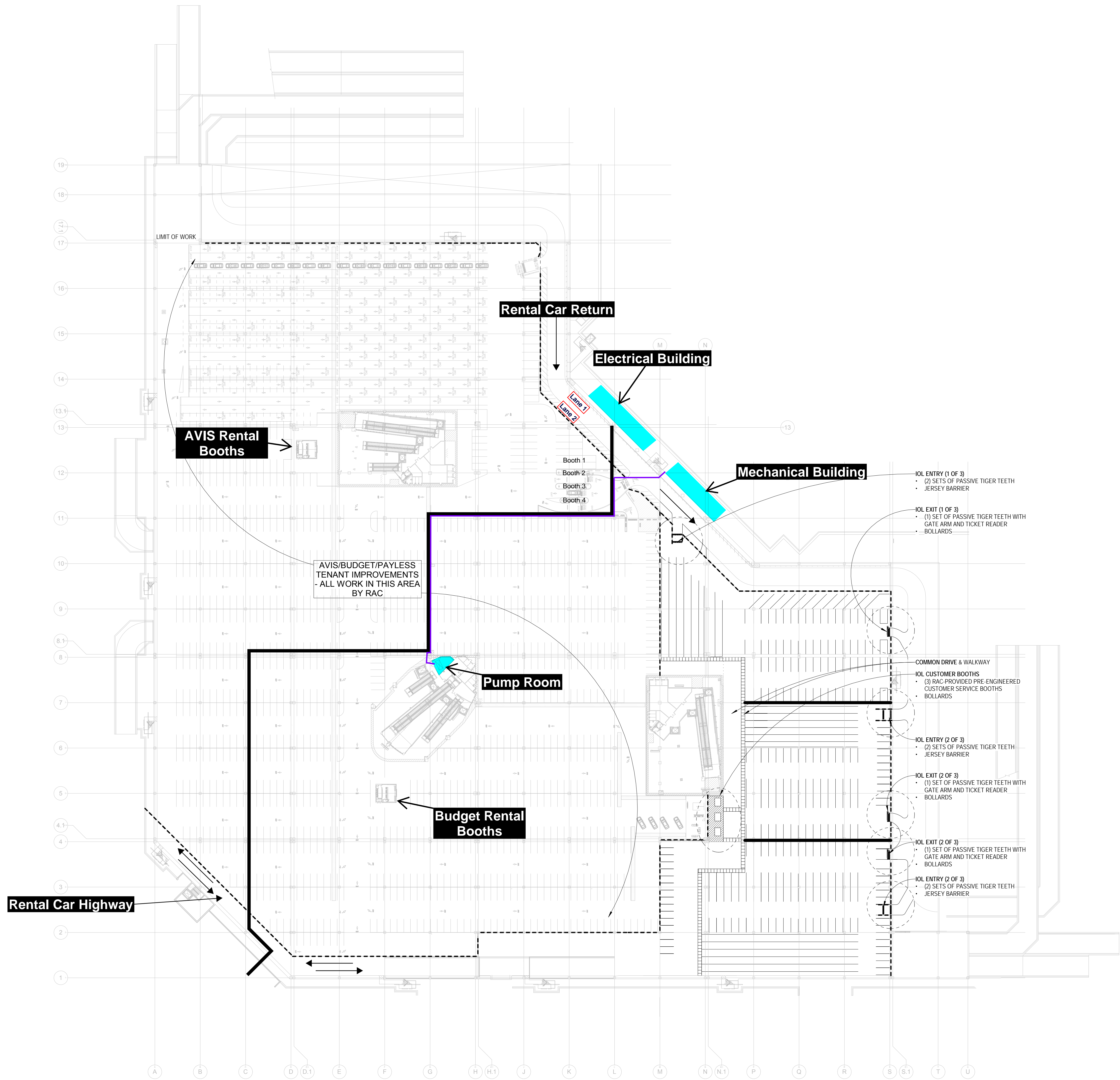
OVERALL GARAGE LEVEL 1 FLOOR PLAN 1/4" = 1'-0" 1
