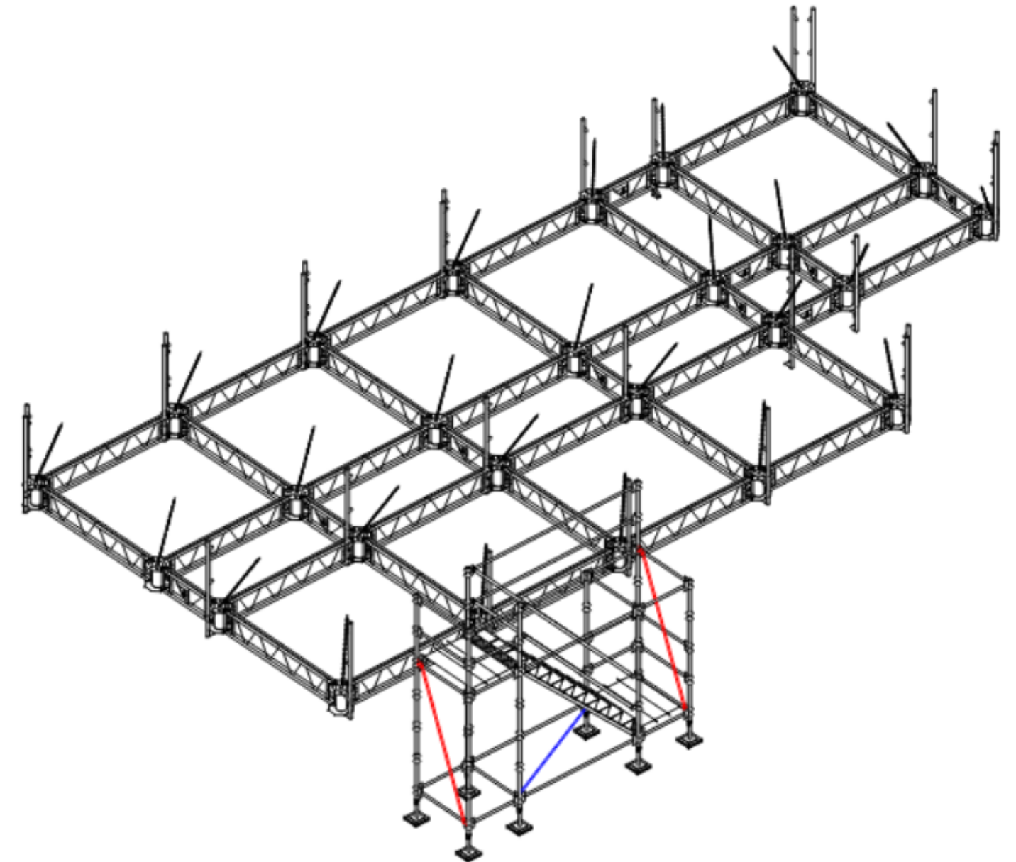
AREA A - ISOMETRIC VIEW
