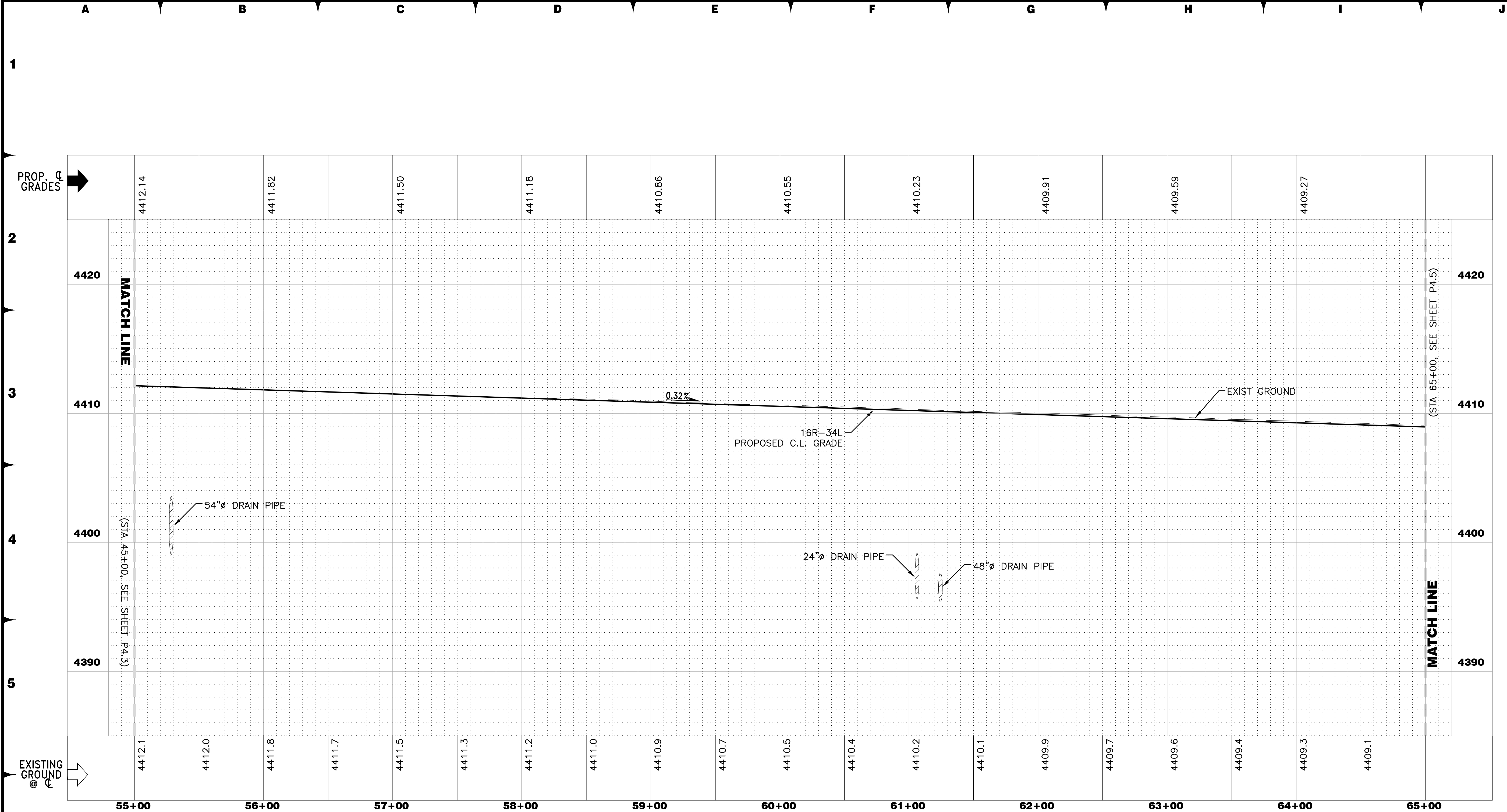
16R-34L CENTERLINE PROFILE
