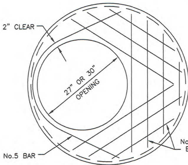
60" DECK PLAN
