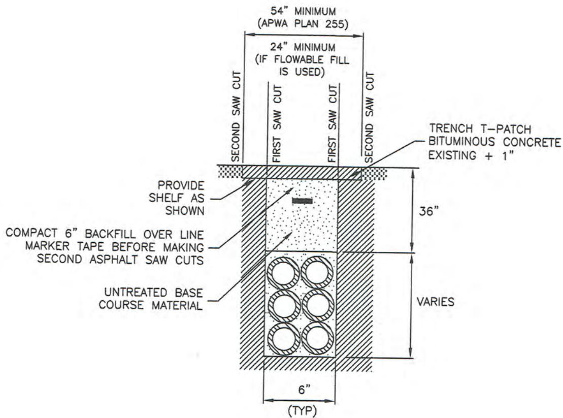
TRENCH DETAIL
