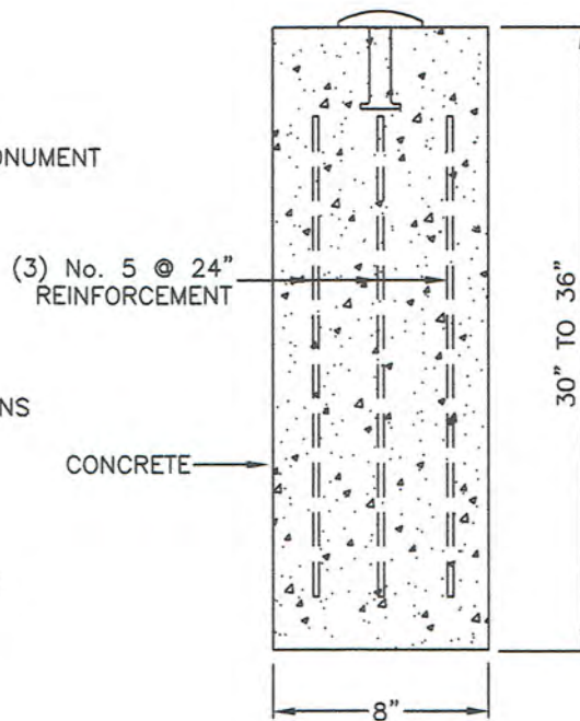
SECTION OF BASE TYPICAL SETTING
