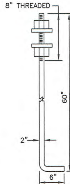
DETAIL B
