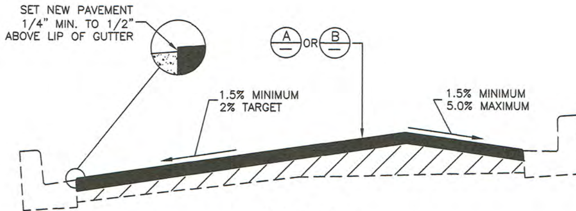
OVERLAY DETAIL
