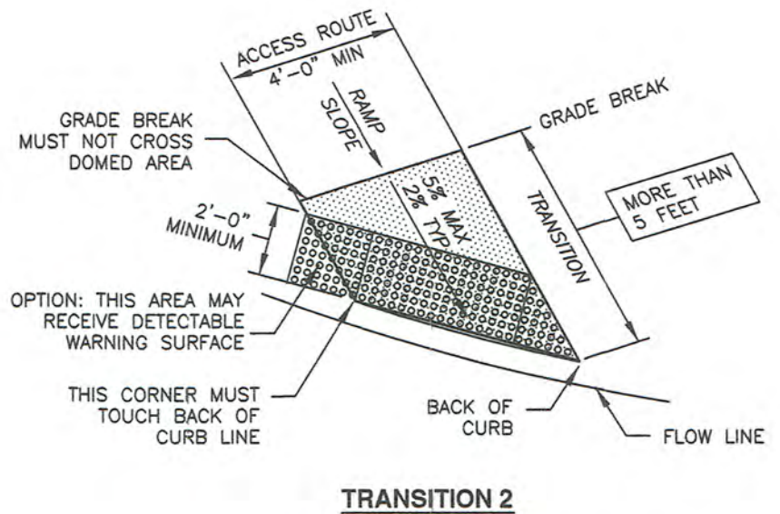
NON-PERPENDICULAR ASSEMBLY
