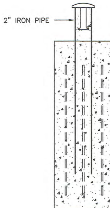
SECTION OF BASE ALTERNATE SETTING
