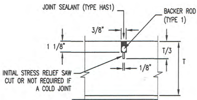
BACKER ROD DETAIL
