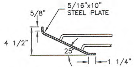
FACE PLATE DETAIL
