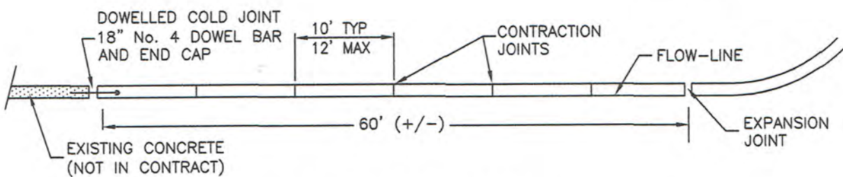
JOINT SPACING DETAIL
