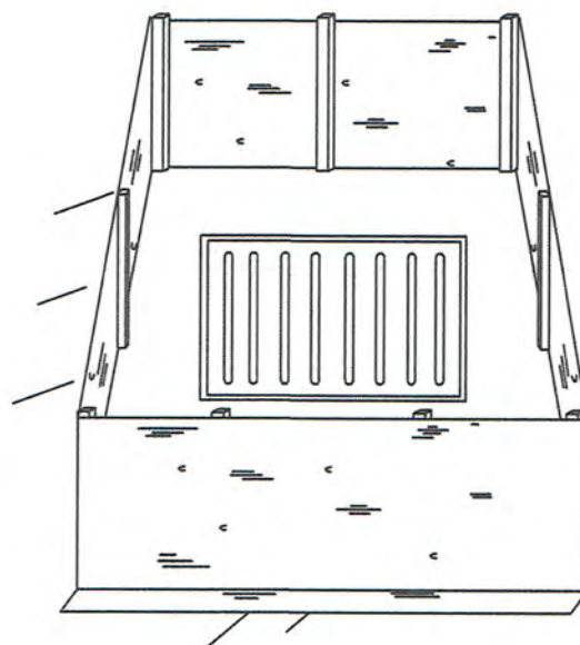
SILT FENCE (Plan No. 121)
