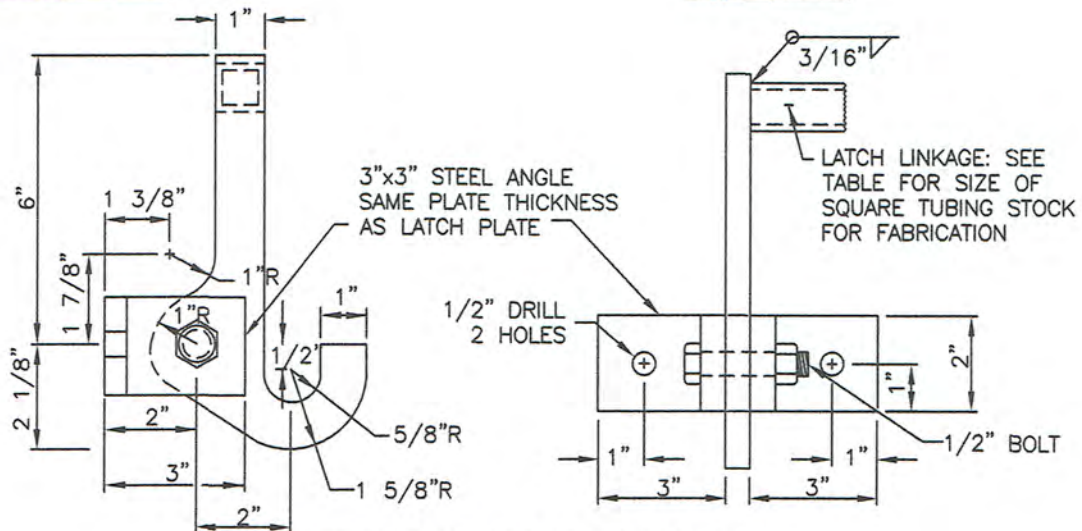
SIDE VIEW
