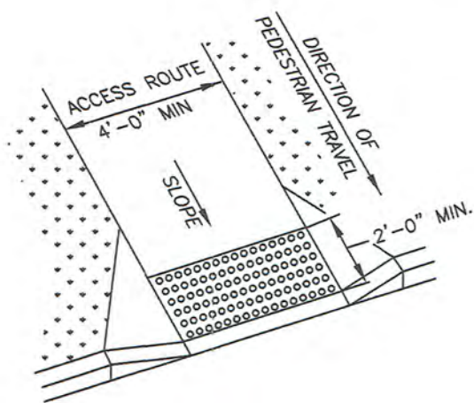
PERPENDICULAR ASSEMBLY
