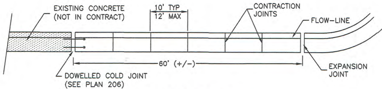
JOINT DETAIL
