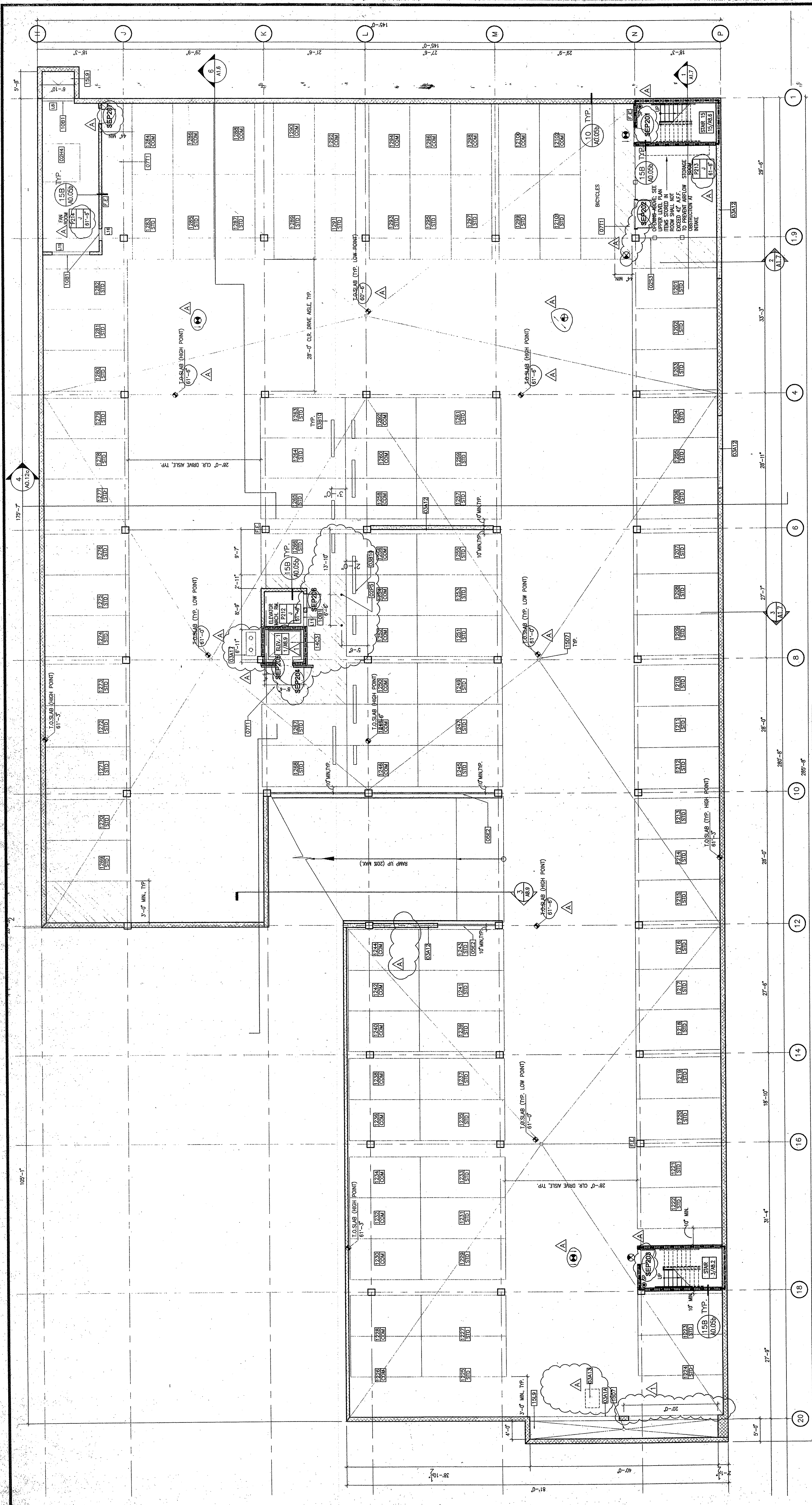
SOUTHEAST GARAGE PLAN (LEVEL P2)
