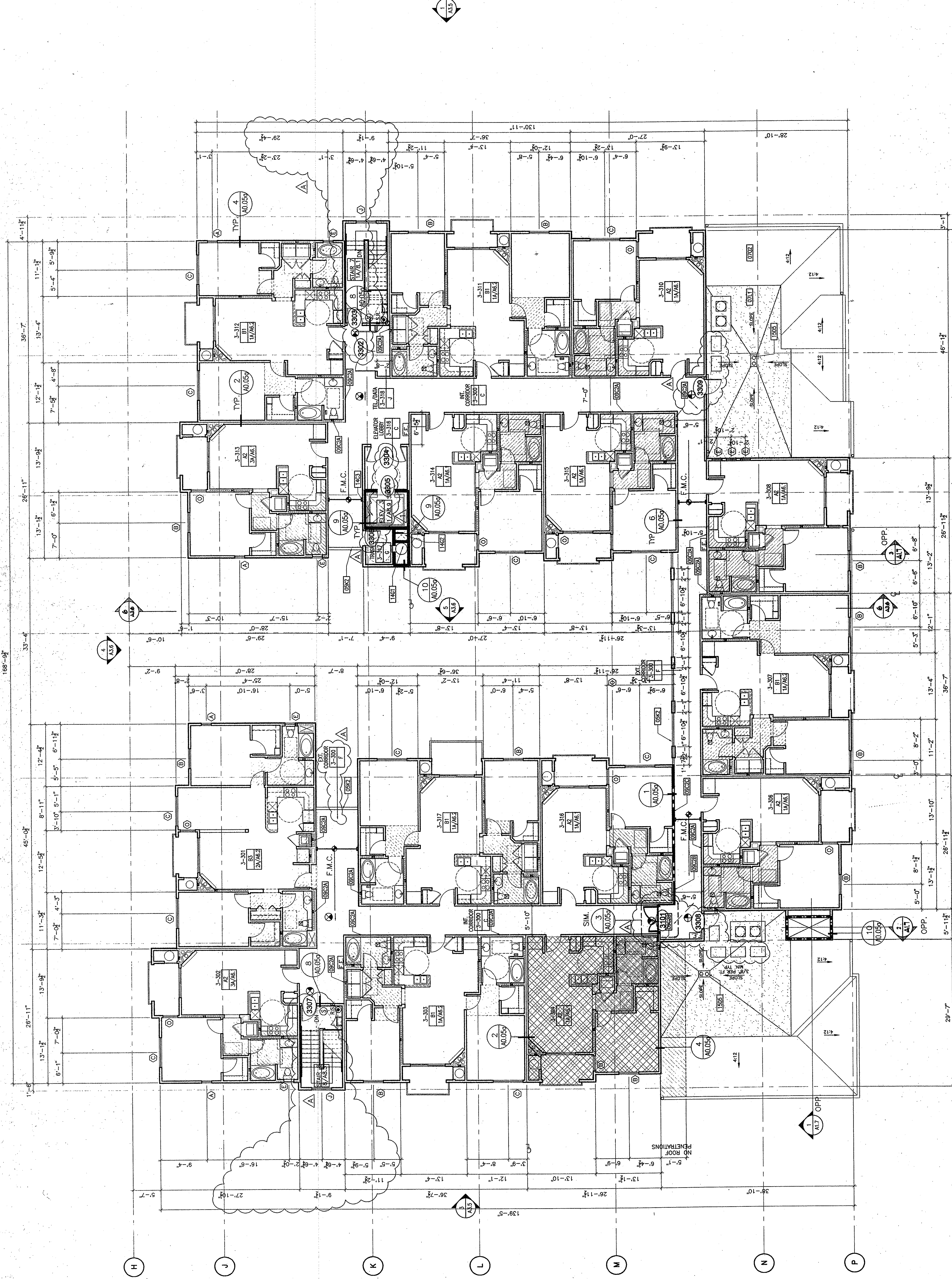
BUILDING THREE - THIRD FLOOR PLAN SCALE: 1/8"=1'-0"
