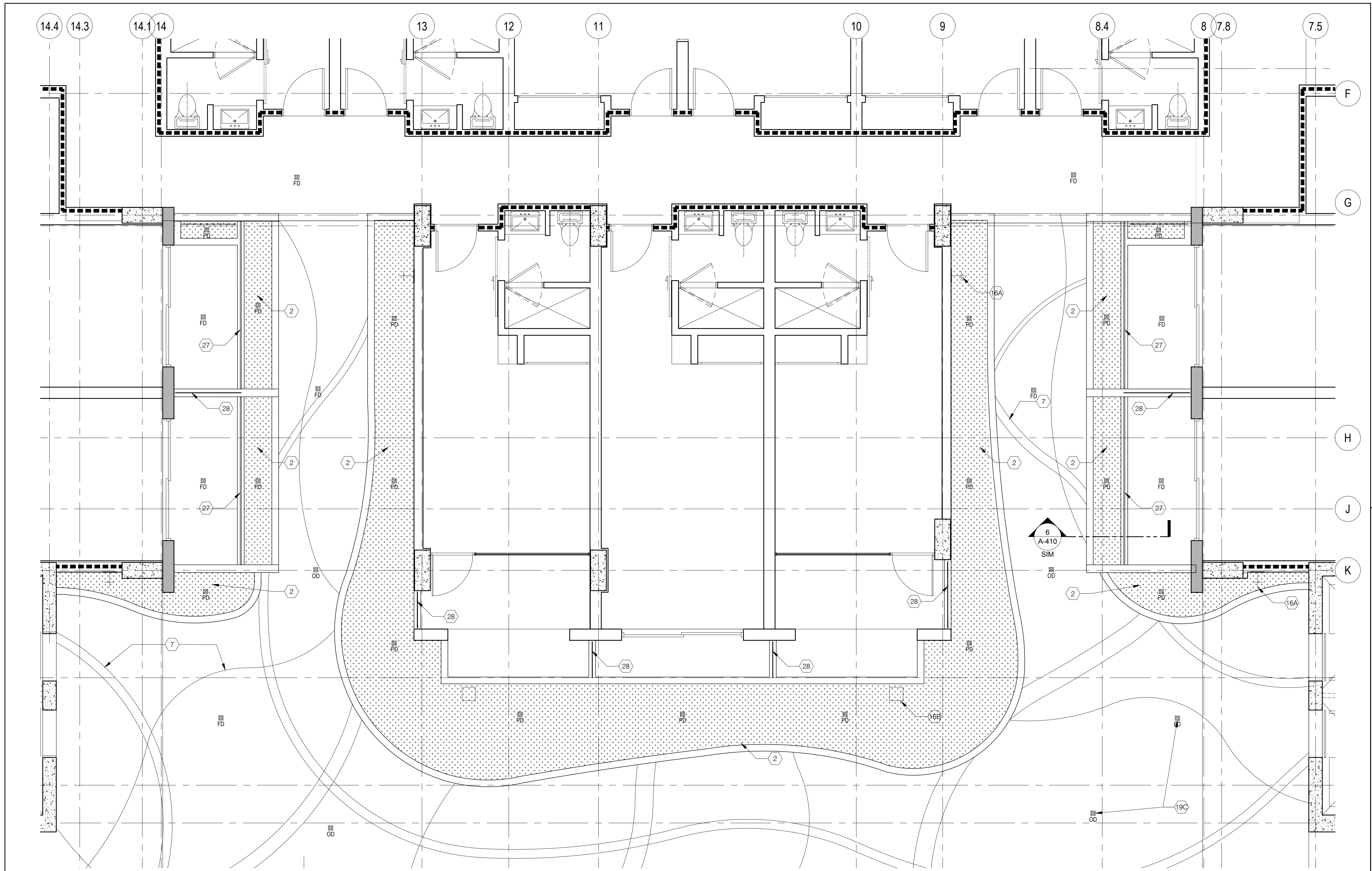
SITE WORK 2ND FLOOR
