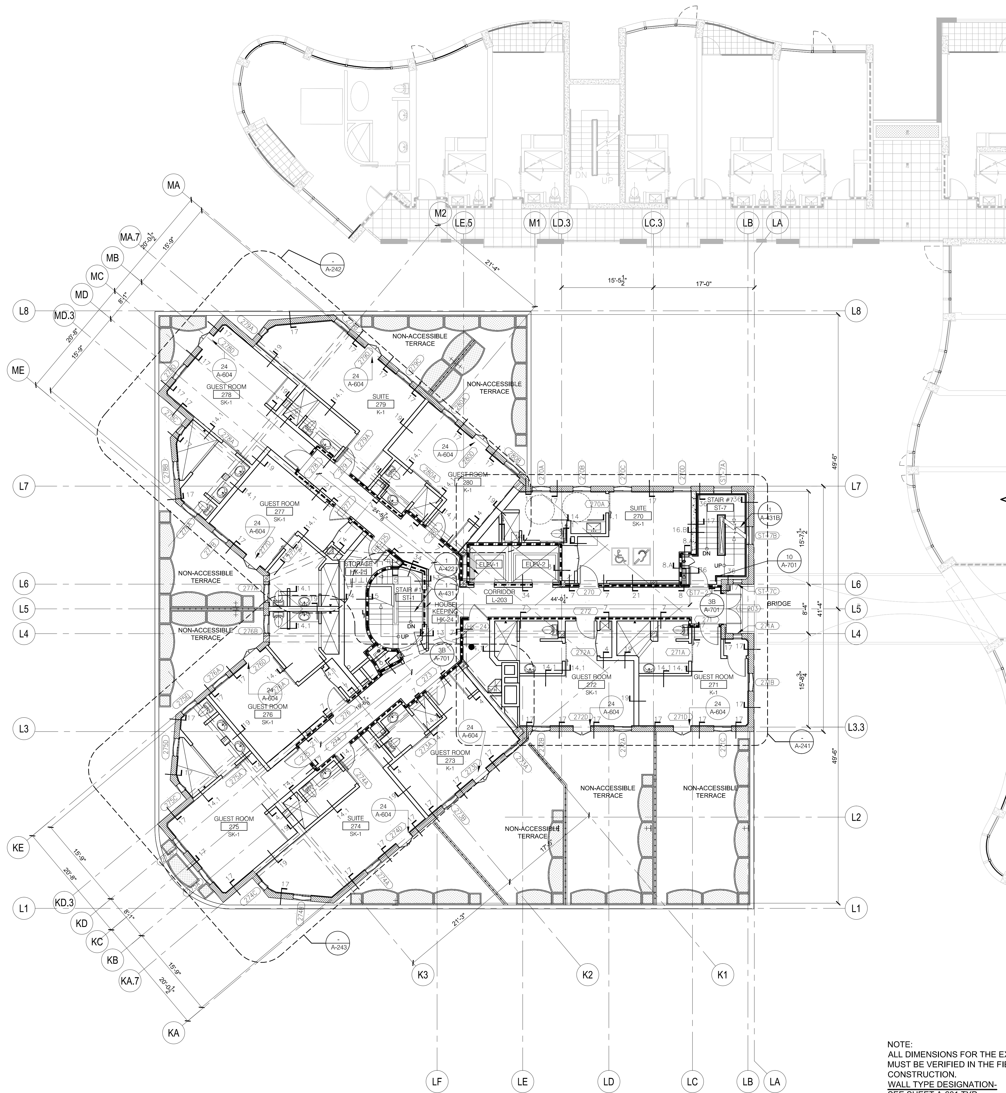
SECOND FLOOR HISTORIC LANDMARK BUILDING REFER TO A-244 FOR FRP & PENETRATION COORDINATION OF 2ND FLOOR
