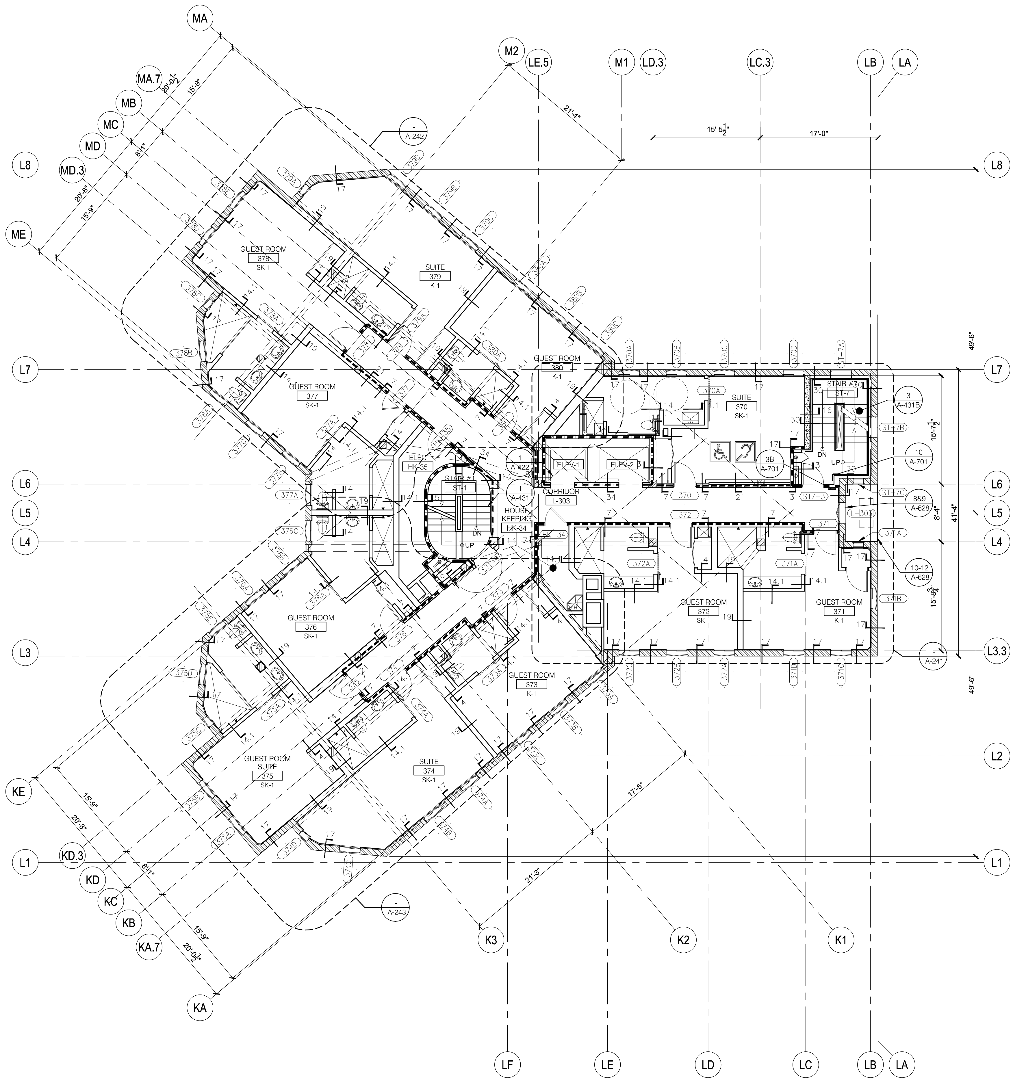
THIRD FLOOR HISTORIC LANDMARK BUILDING
