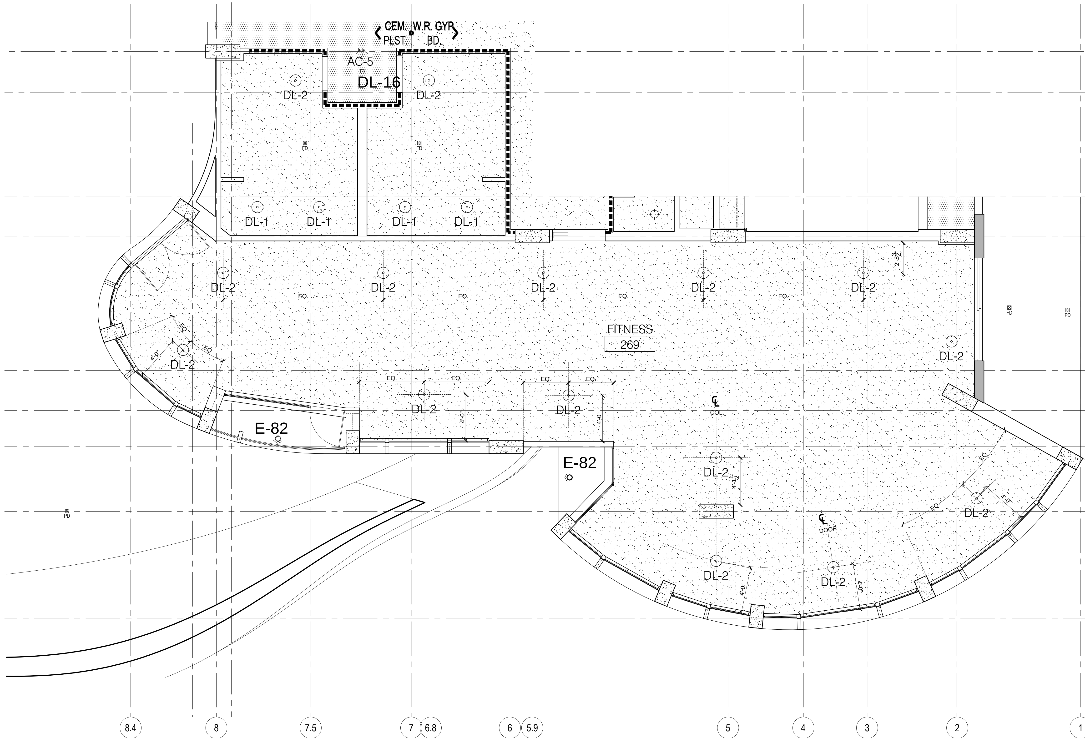
ENLARGED PLAN FOR FITNESS ROOM, MENS & WOMENS TOILET
