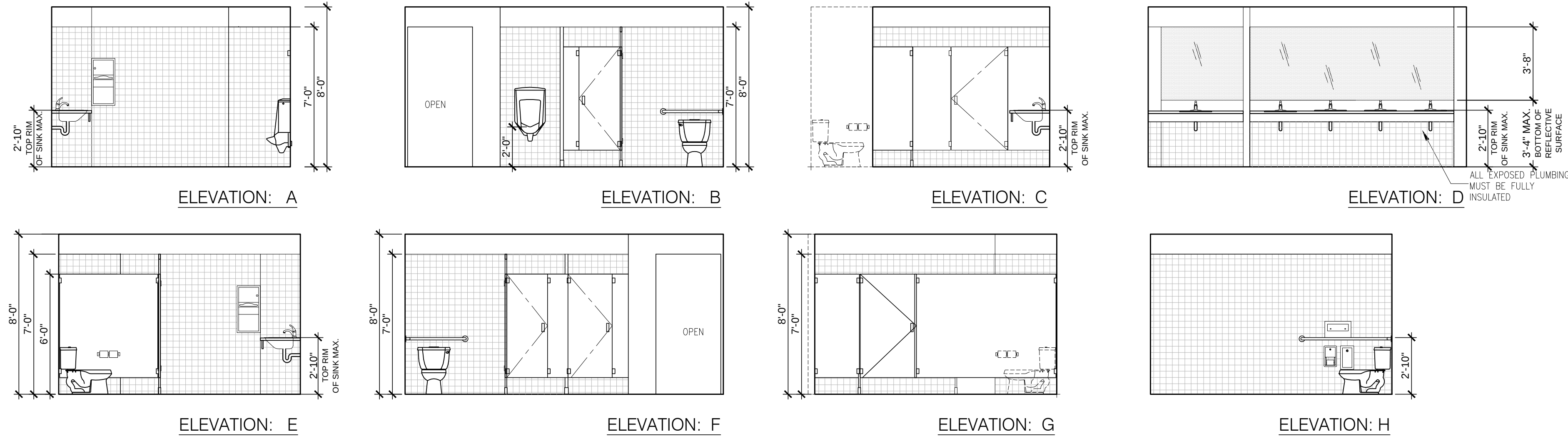
TOILET ROOM ELEVATIONS
