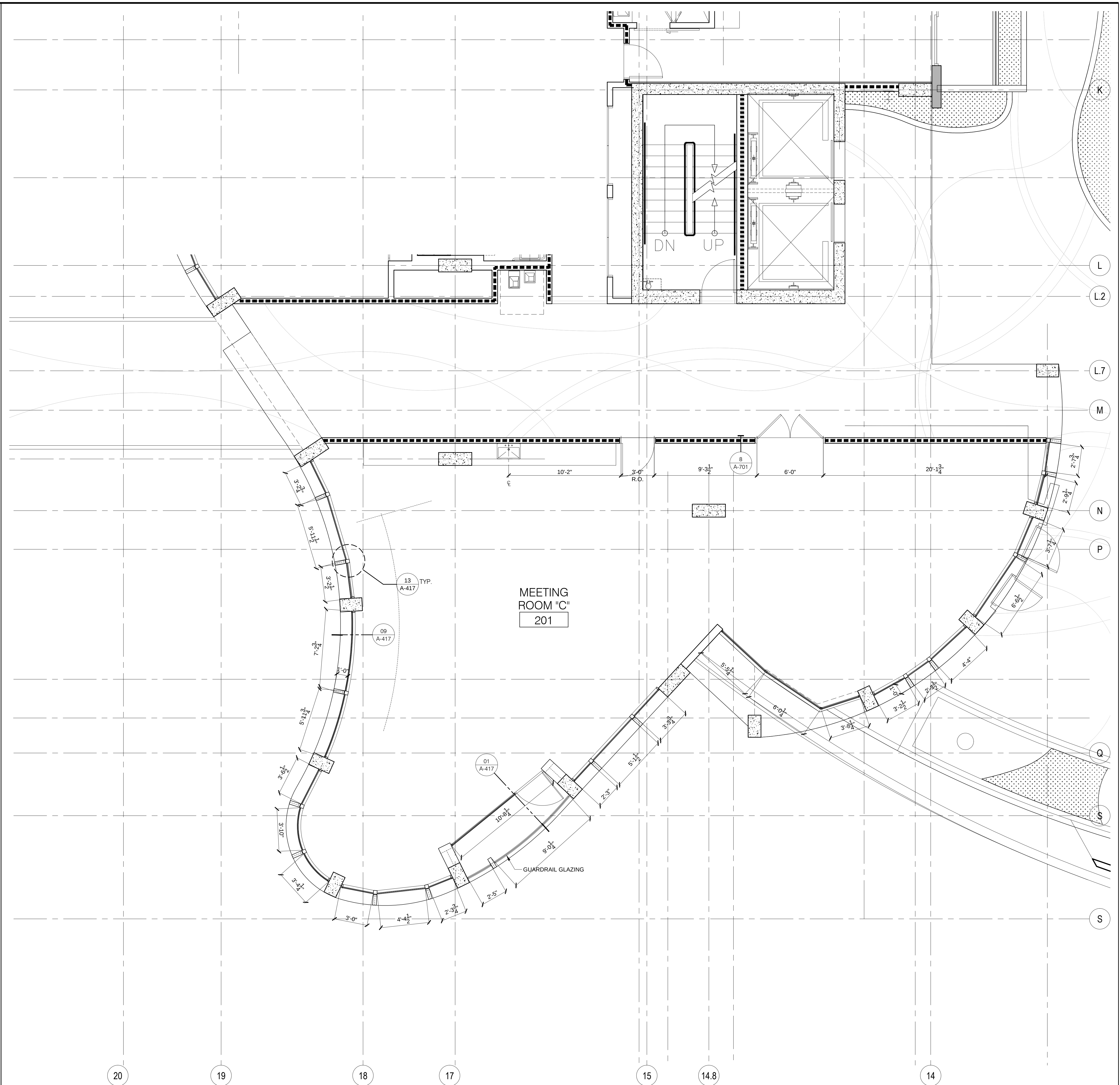
ENLARGED PLAN OF MEETING ROOM
