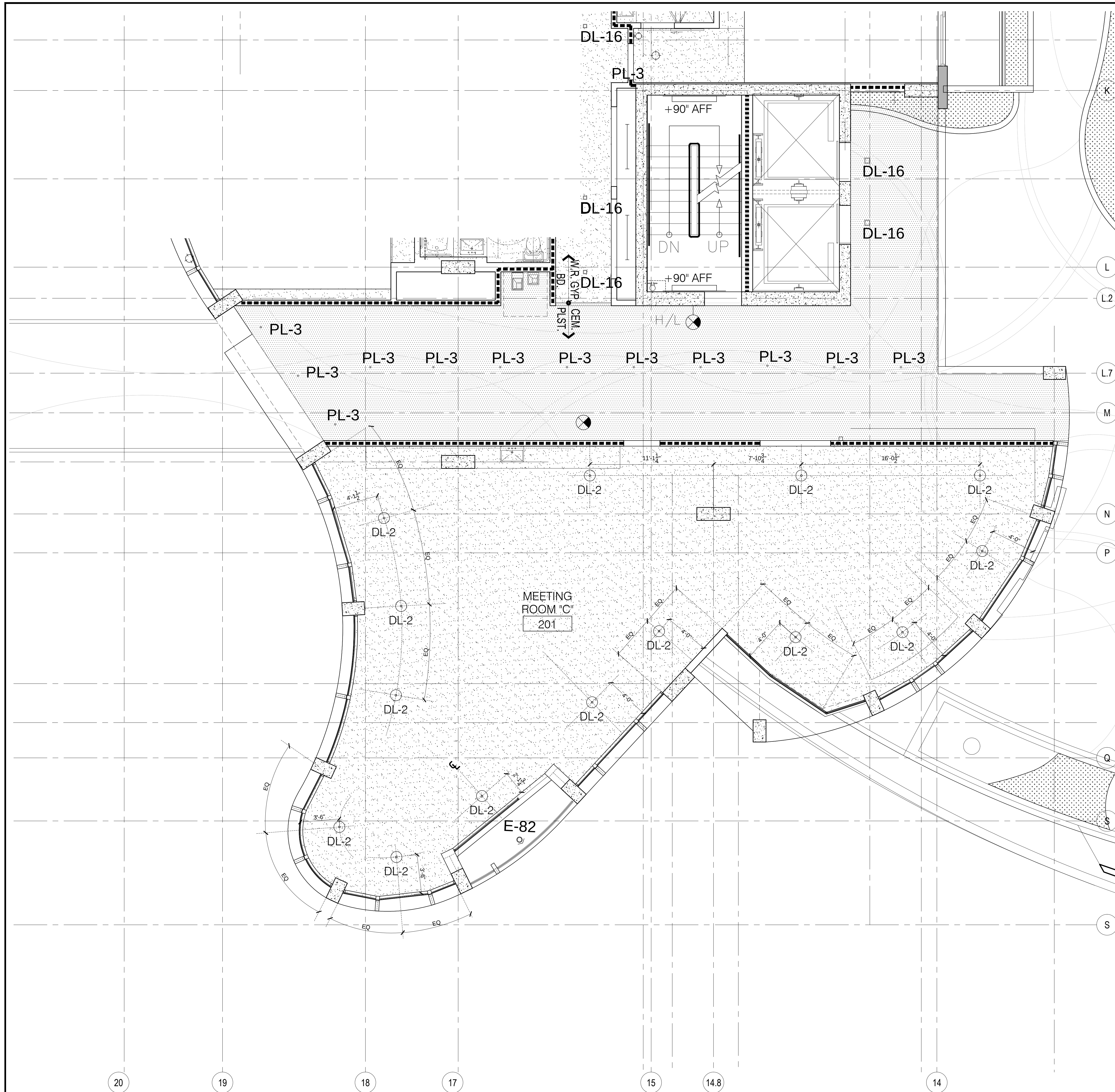
ENLARGED RCP PLAN OF MEETING ROOM
