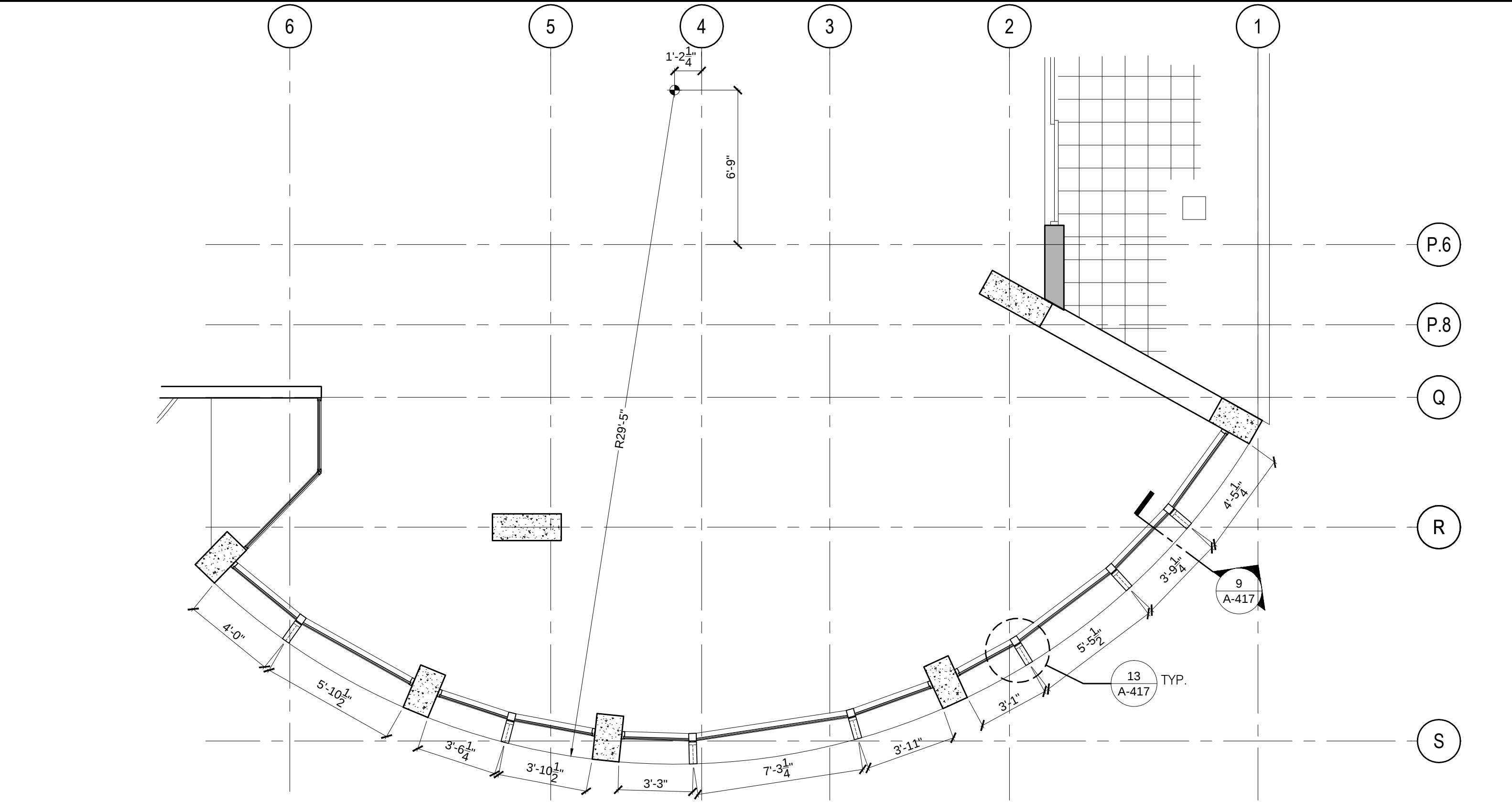
ENLARGED PLAN - LEVEL 02
