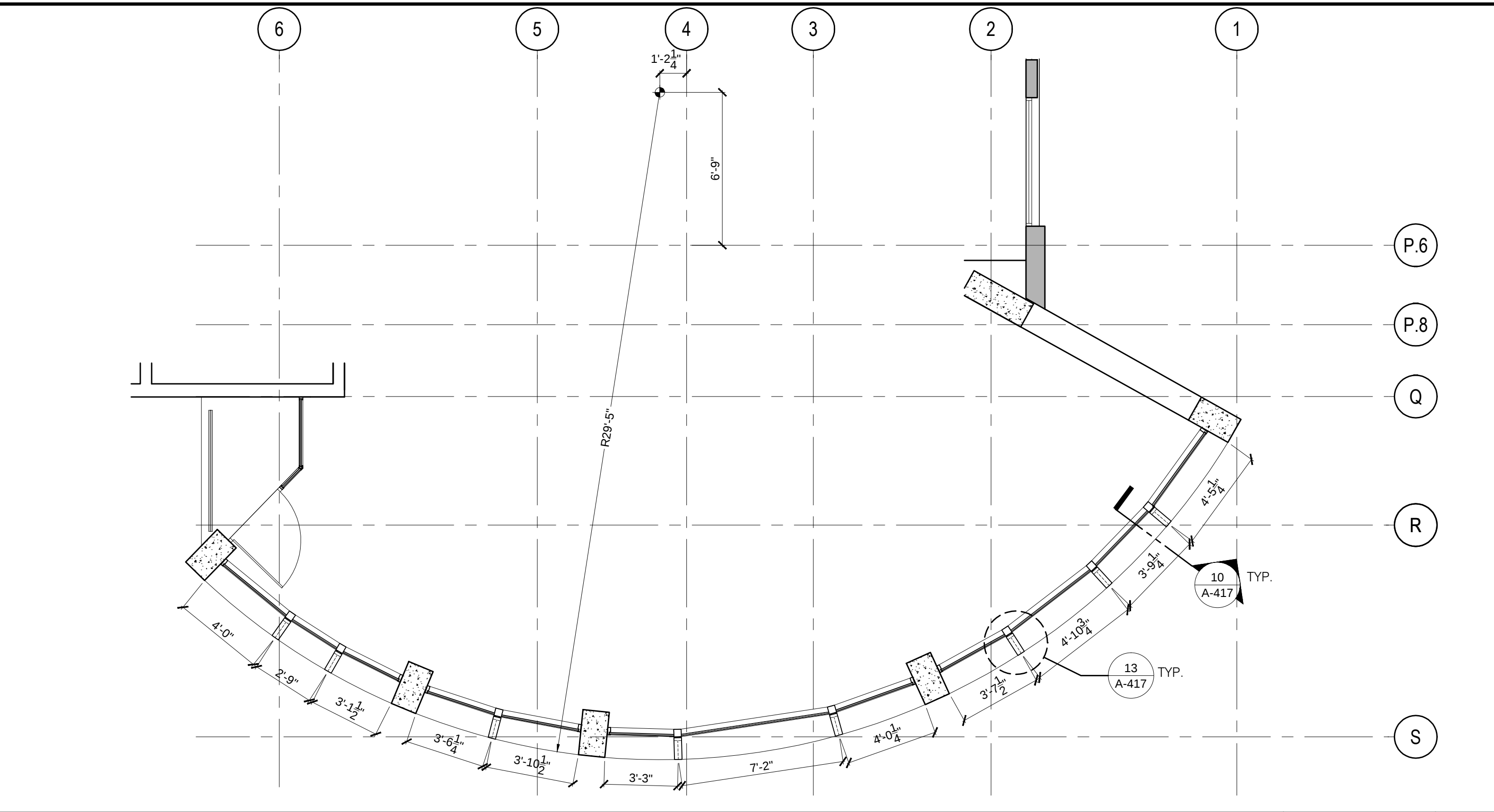
ENLARGED PLAN - LEVEL 06
