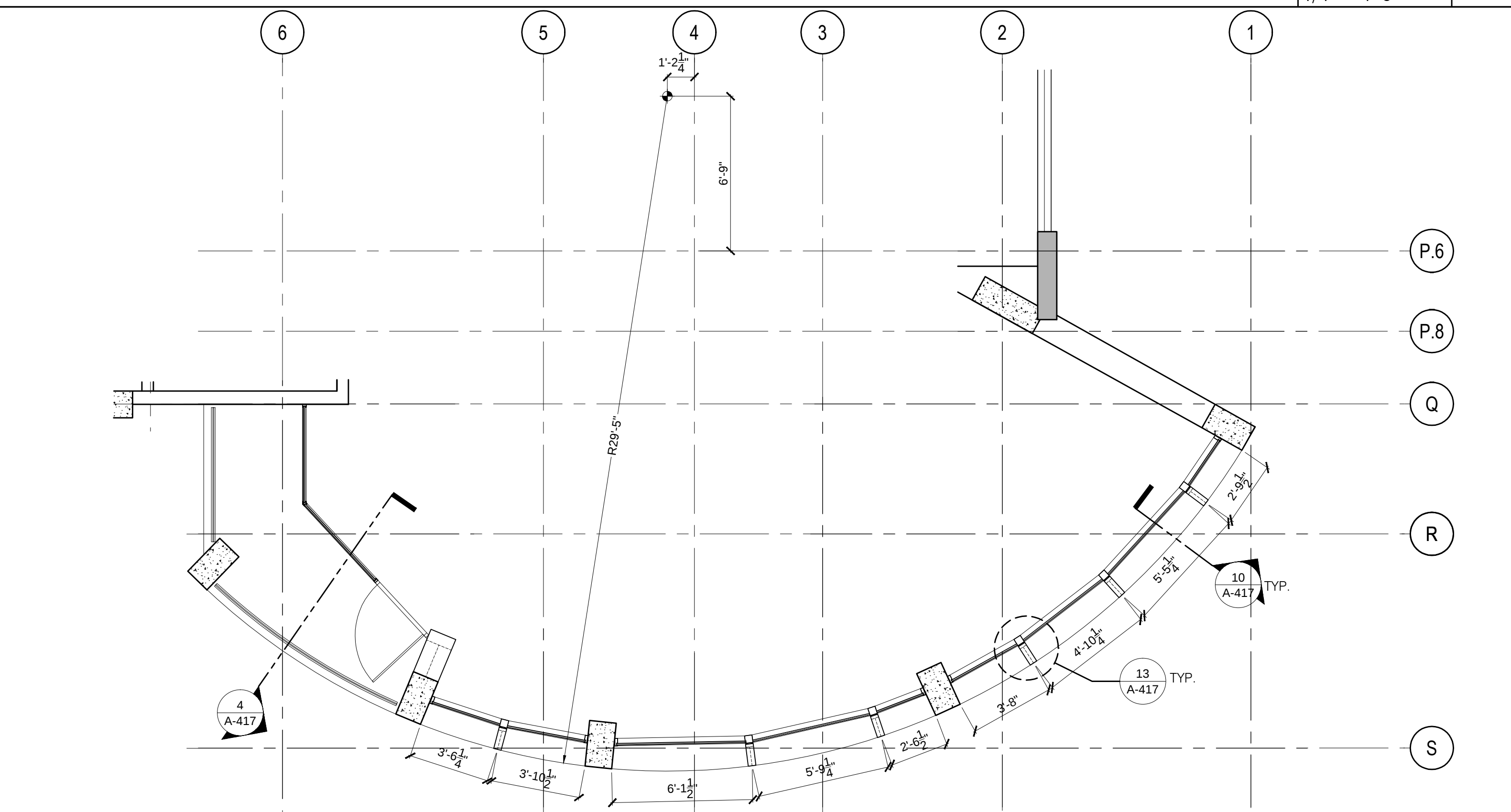
ENLARGED PLAN - LEVEL 04
