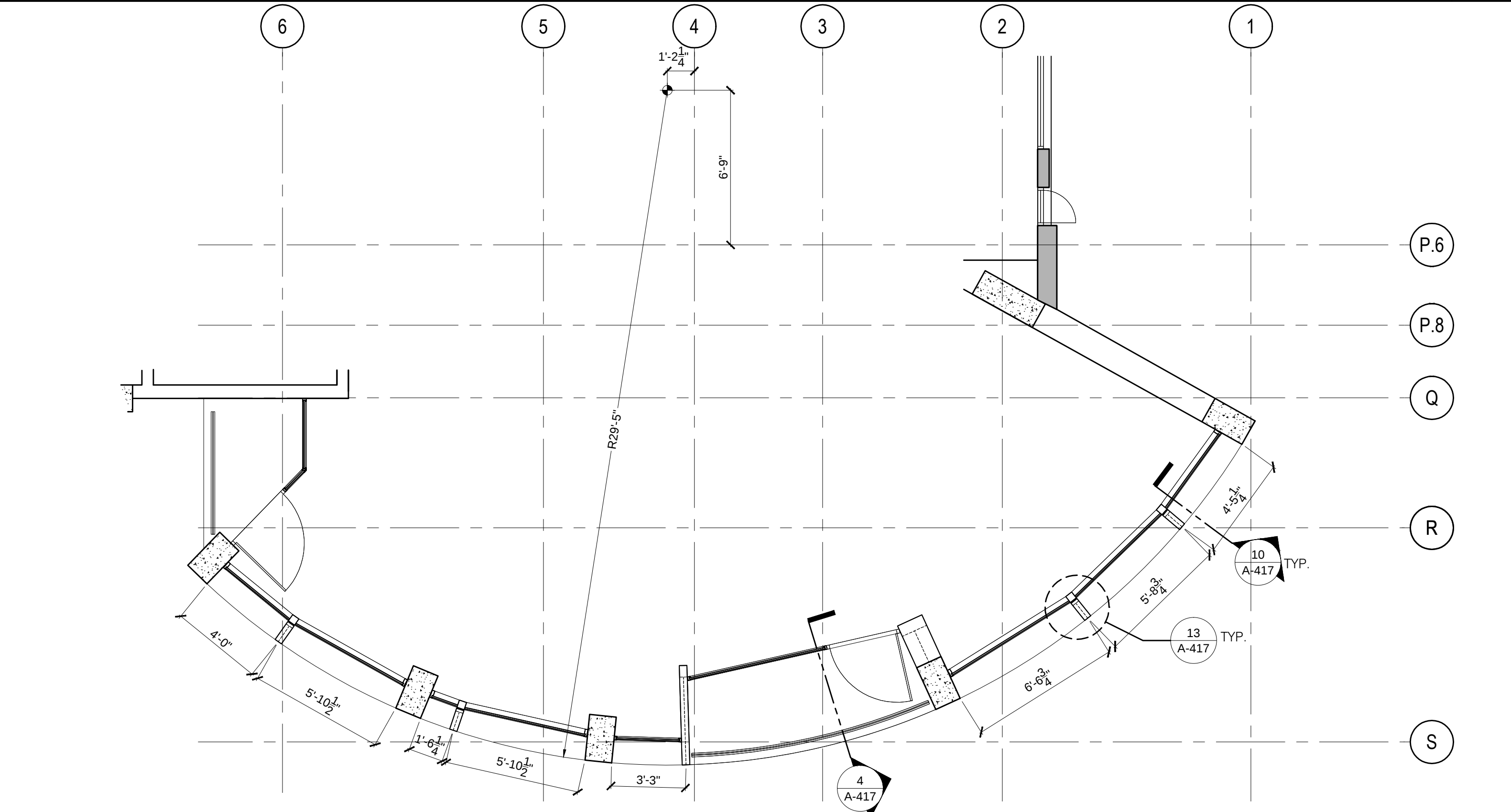
ENLARGED PLAN - LEVEL 05
