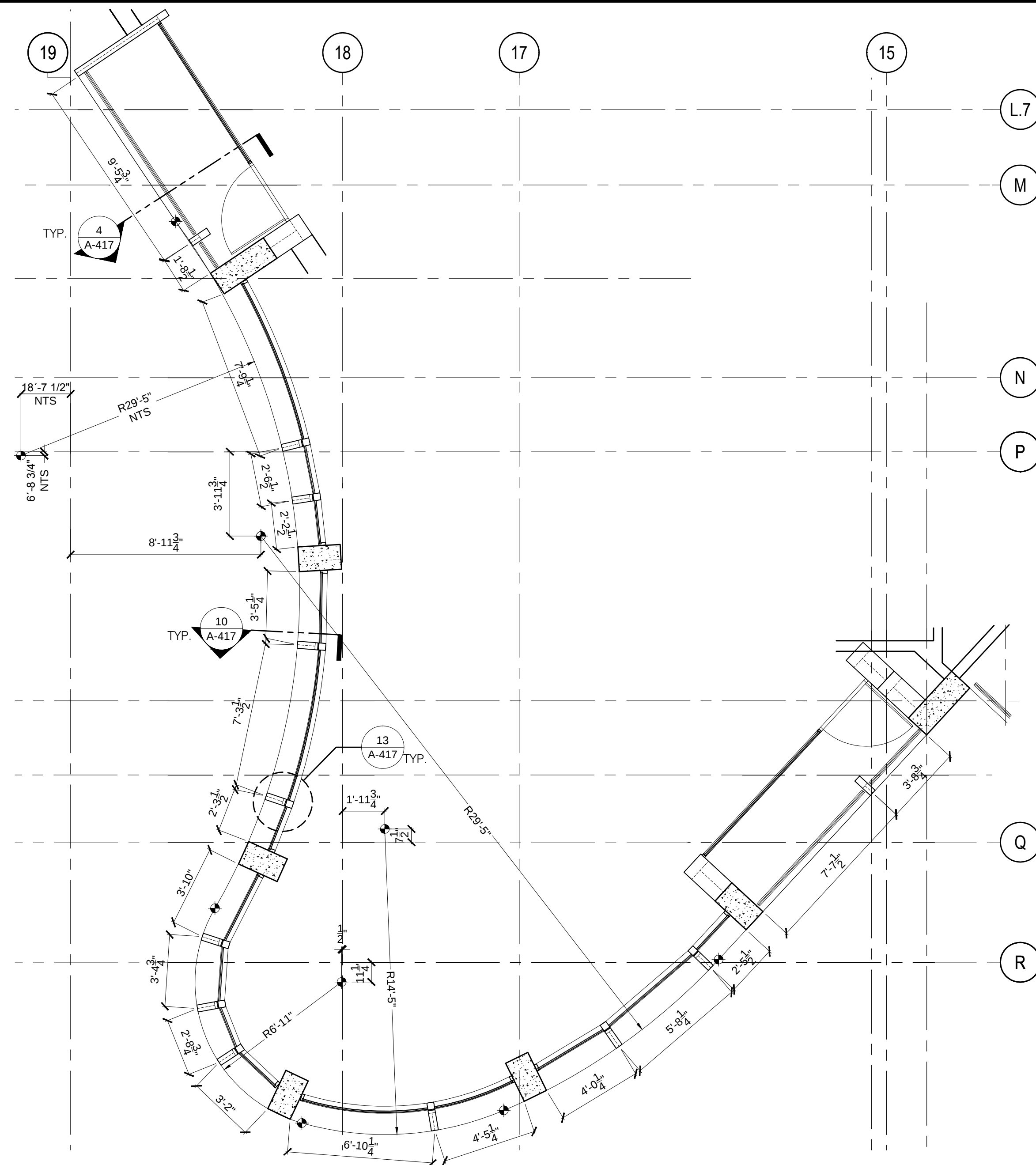
ENLARGED PLAN - LEVEL 04
