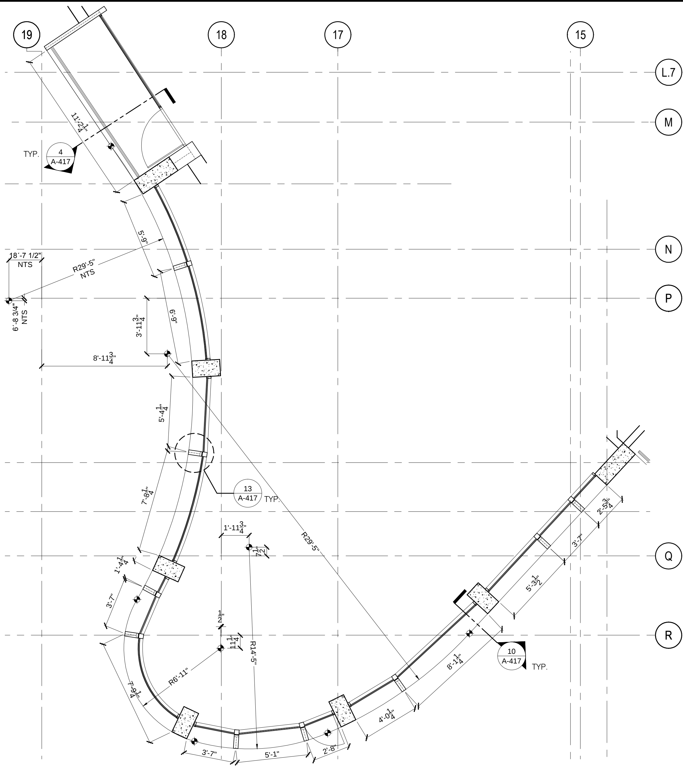
ENLARGED PLAN - LEVEL 06
