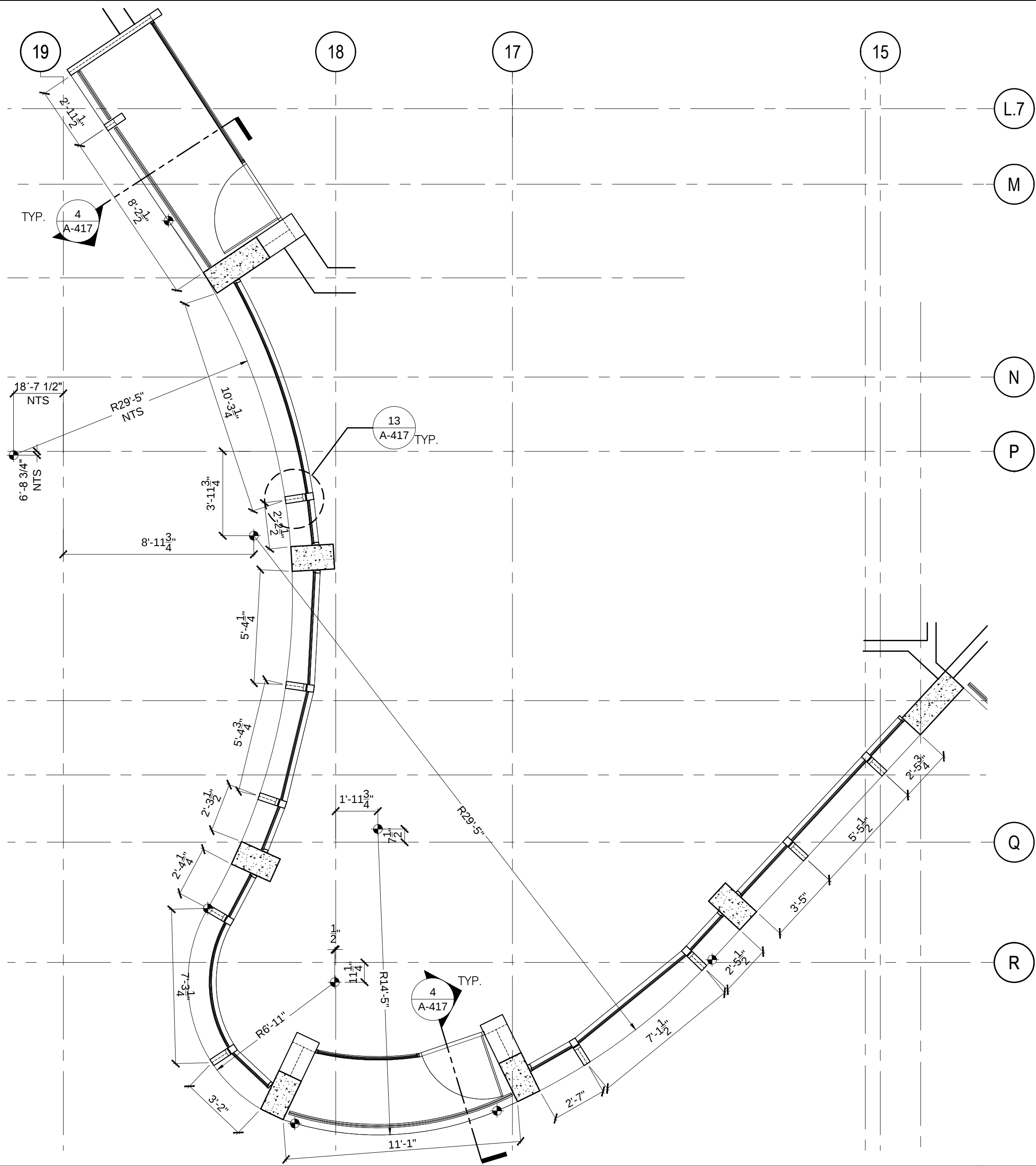
ENLARGED PLAN - LEVEL 05
