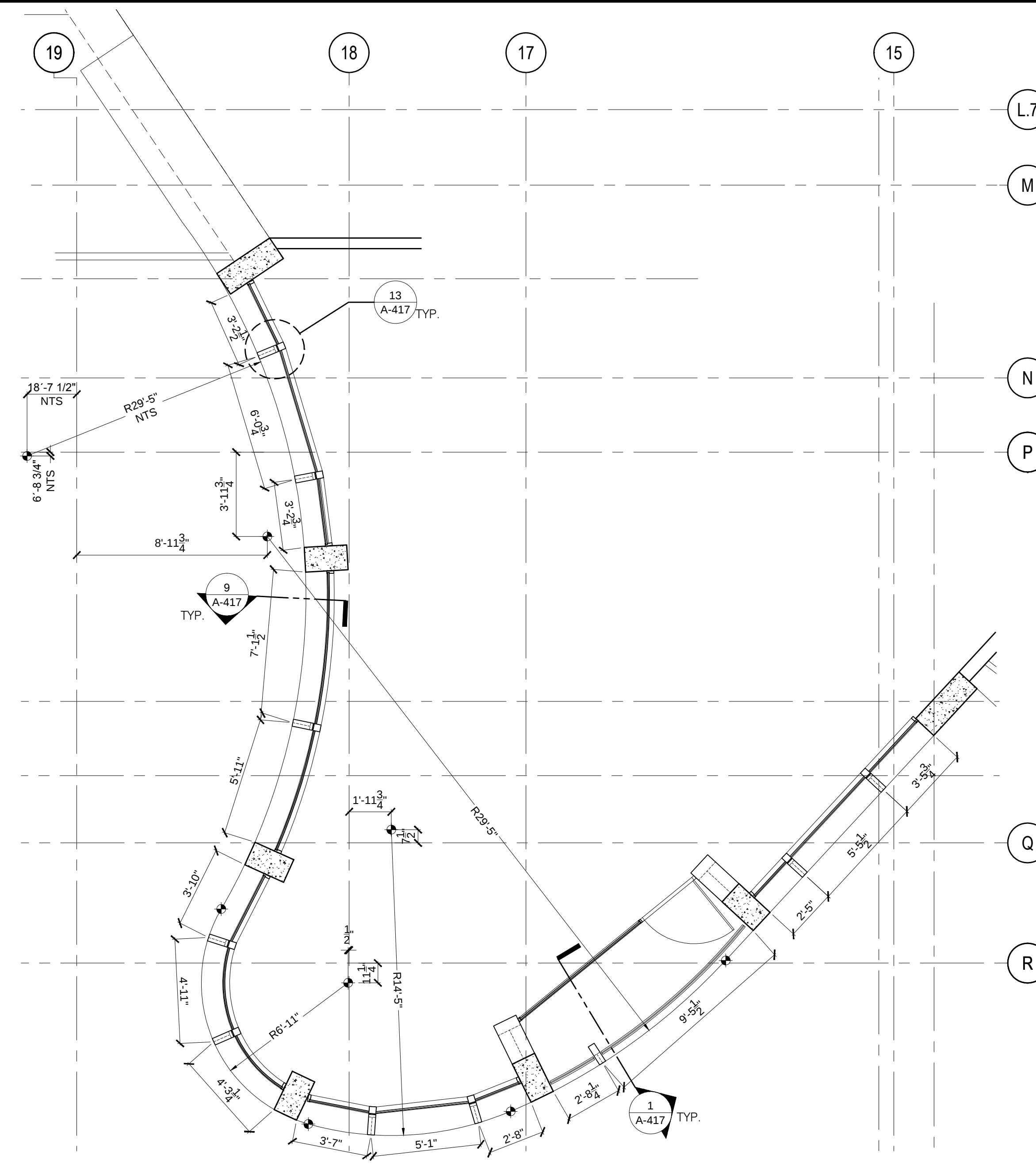
ENLARGED PLAN - LEVEL 02
