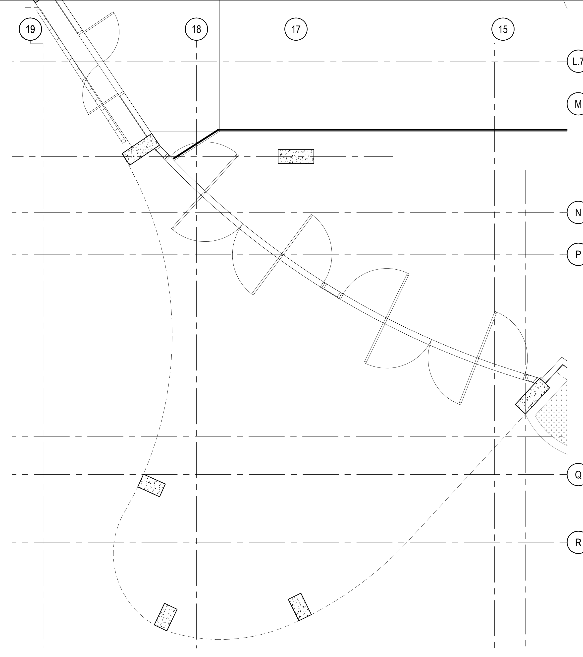
ENLARGED PLAN - GROUND LEVEL
