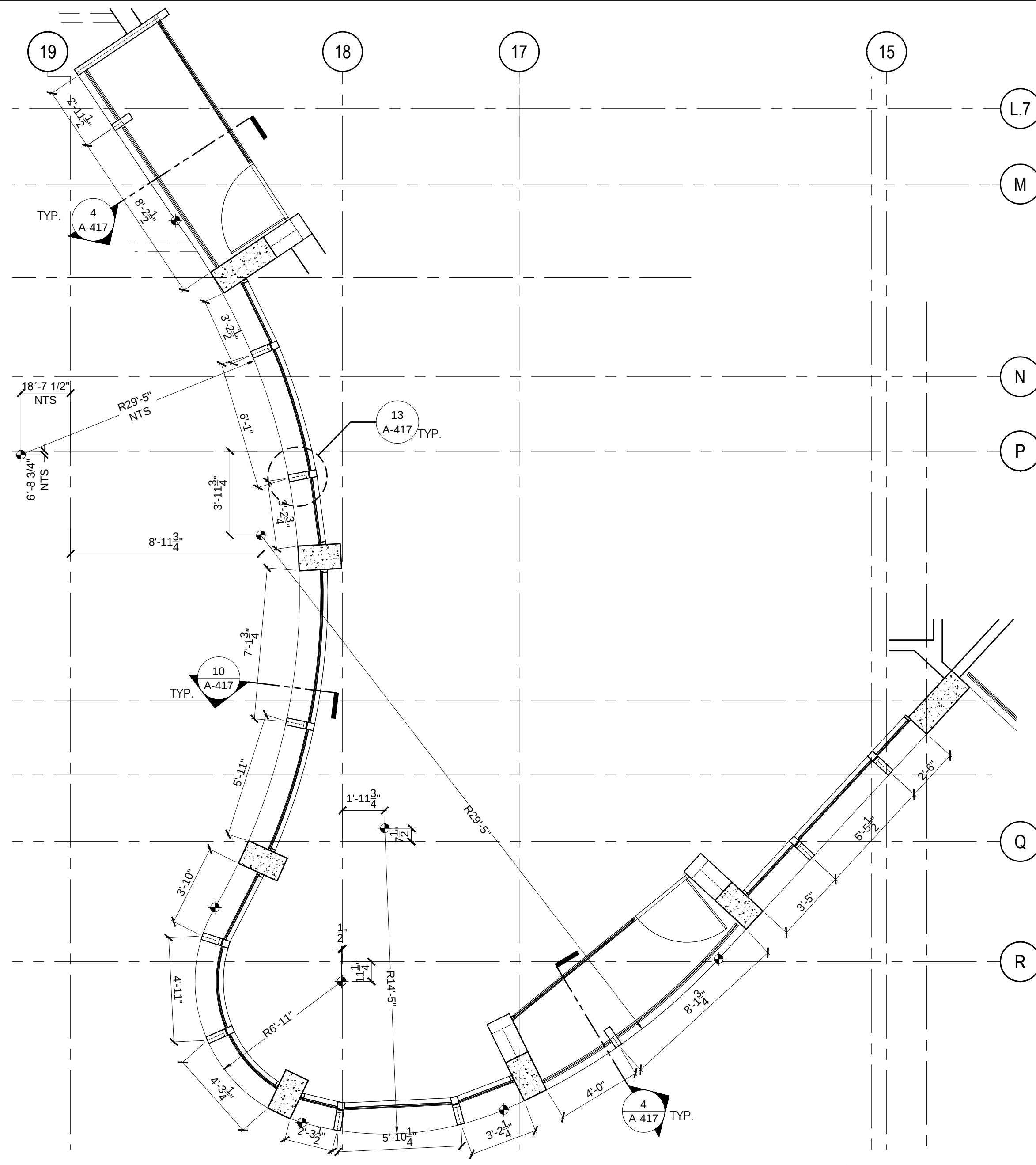
ENLARGED PLAN - LEVEL 03
