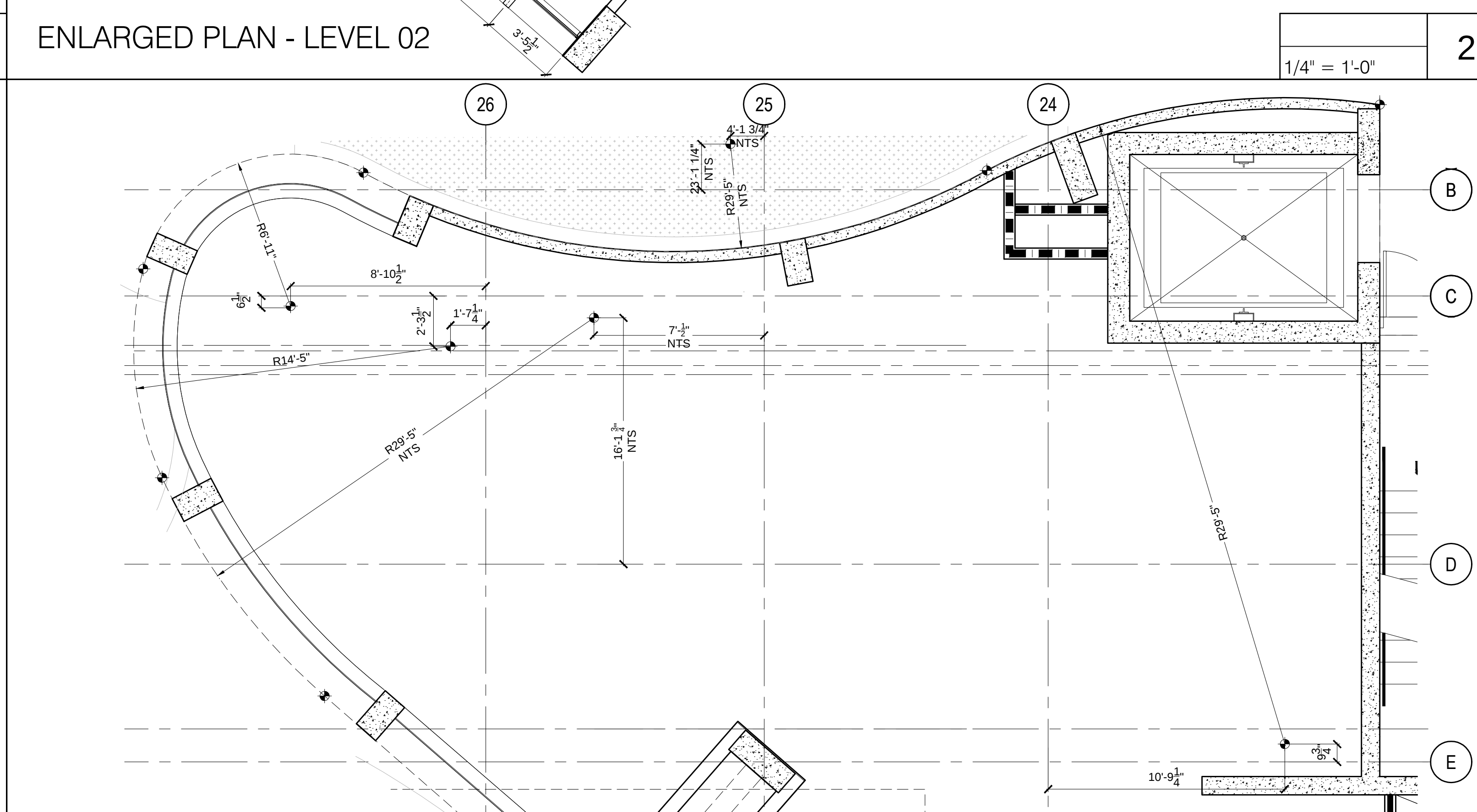
ENLARGED PLAN - GROUND LEVEL
