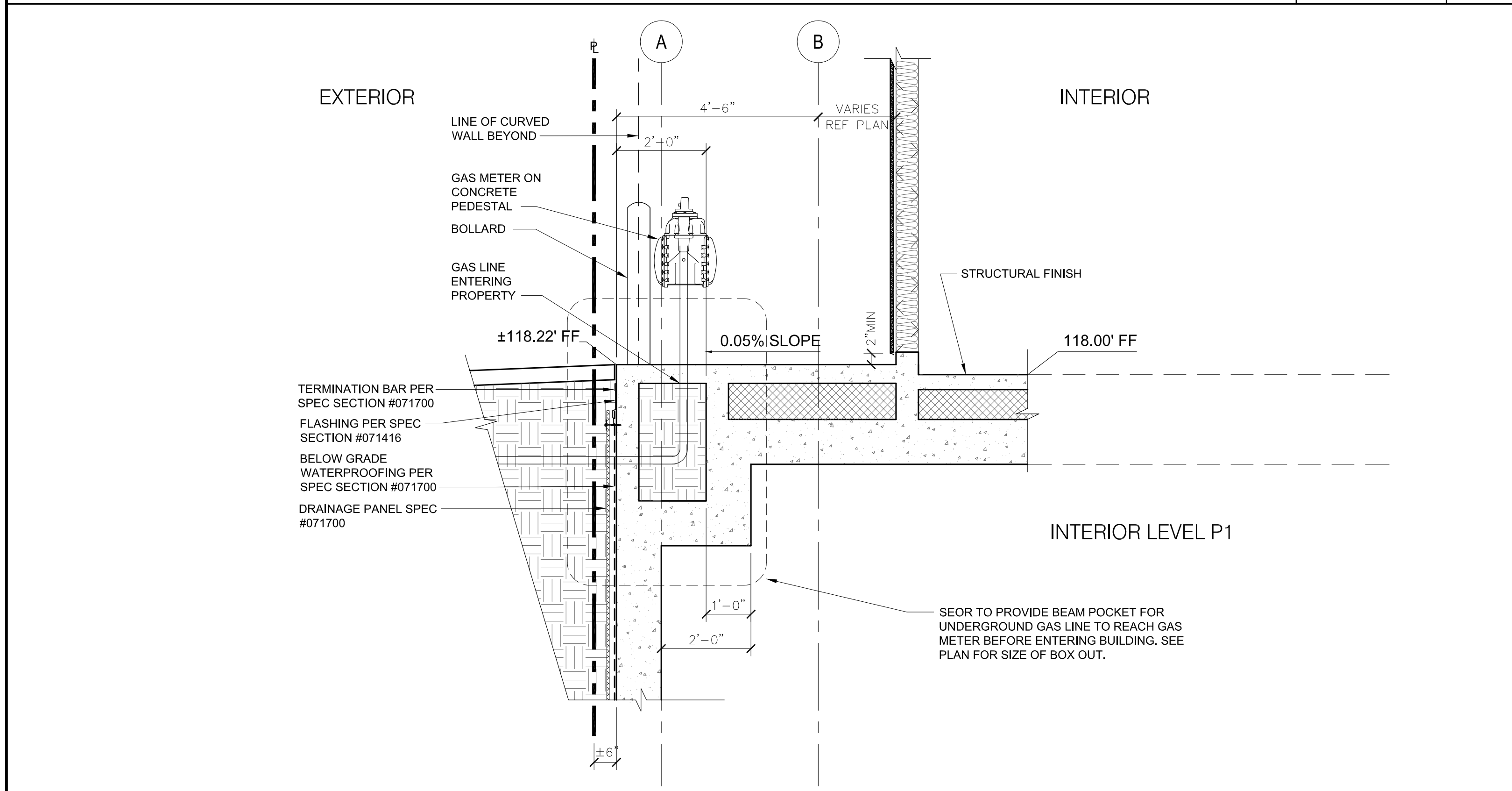
GAS METER PEDESTAL SECTION
