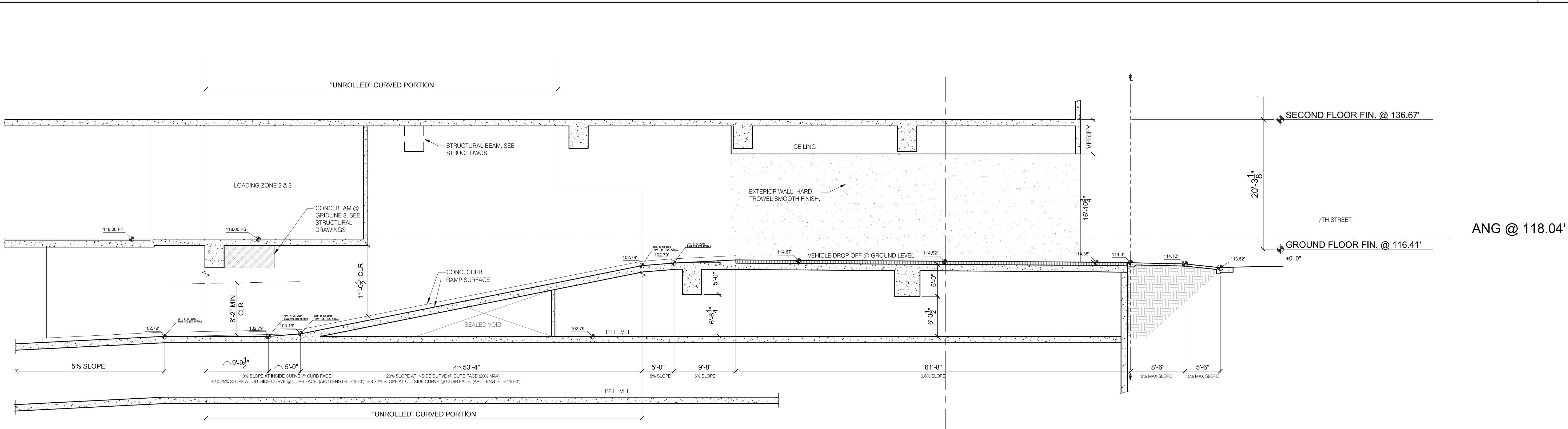
"UNROLLED" VEHICLE RAMP GROUND TO P1 SECTION
