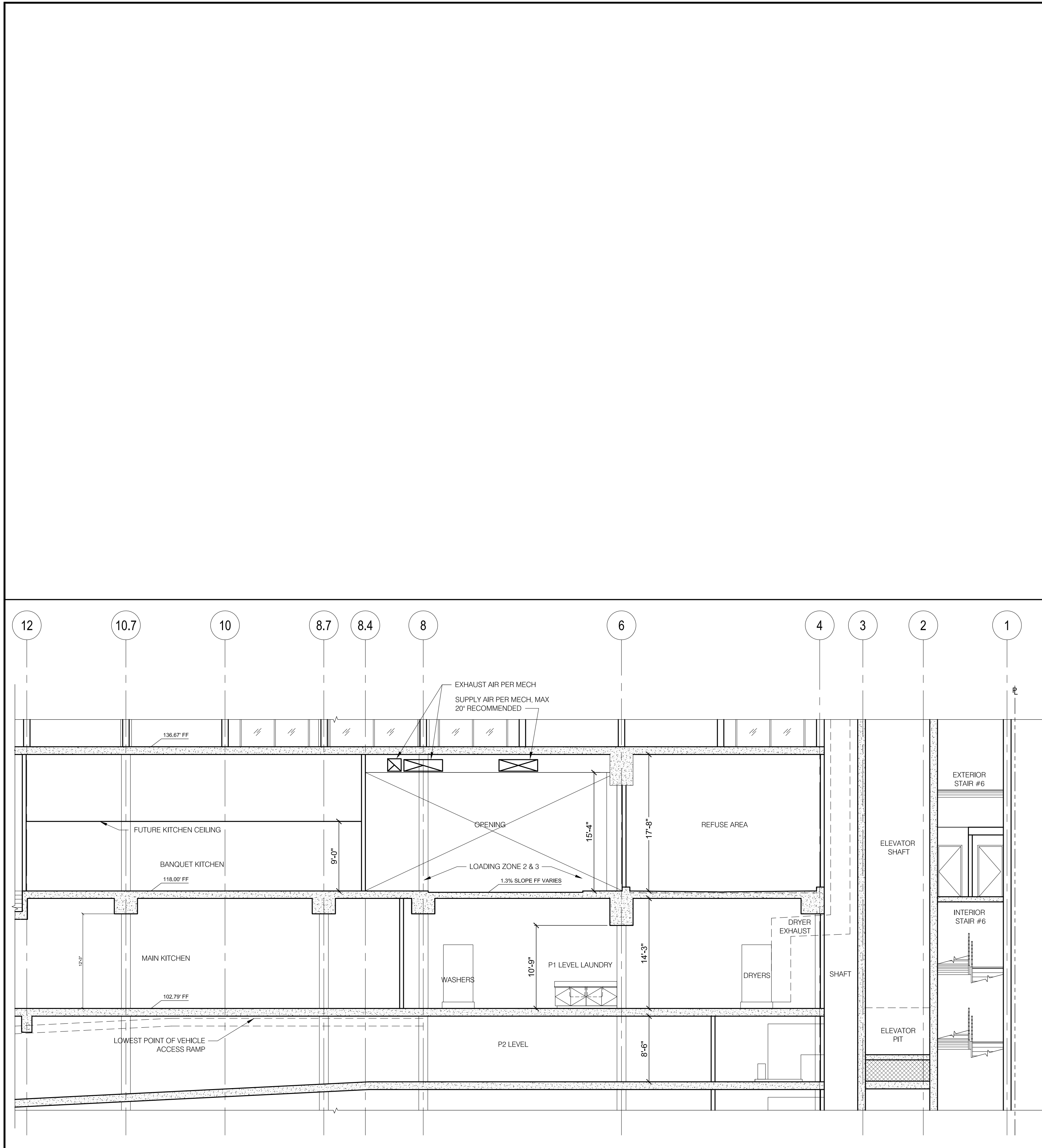
SECTION AT KITCHEN TO EXHAUST
