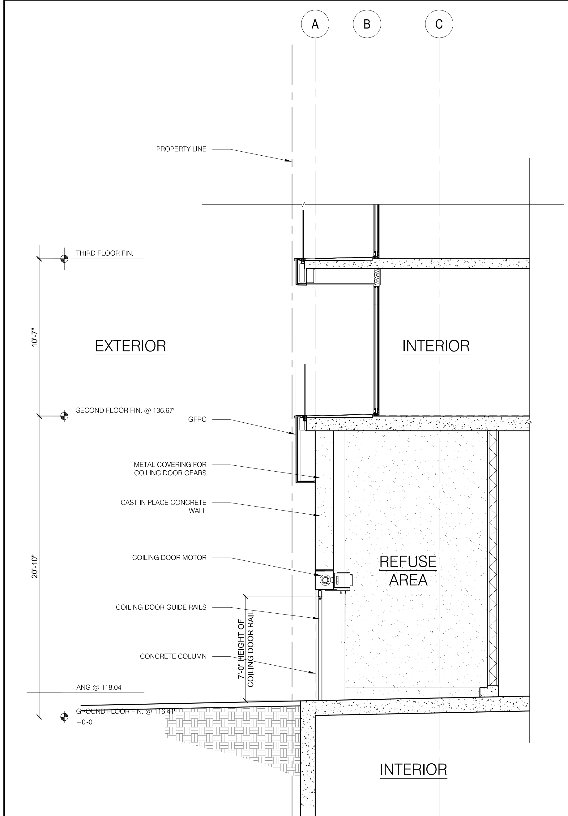
SECTION AT ALLEY REFUSE AREA
