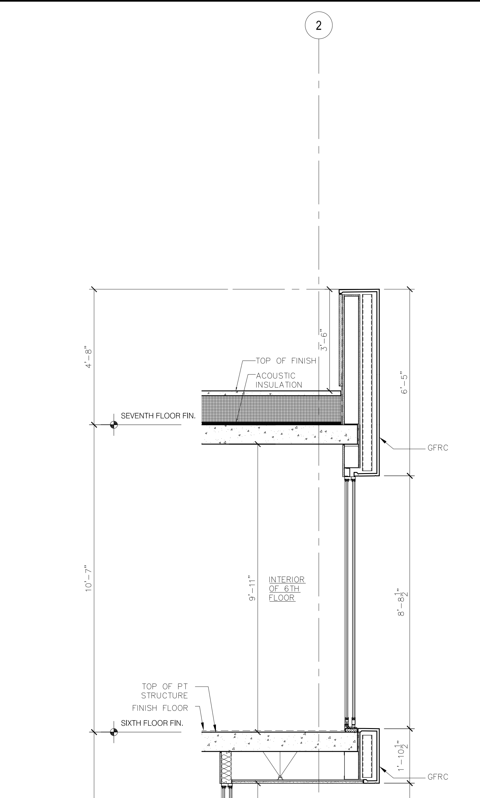
WALL SECTION @ SOUTH TOWER
