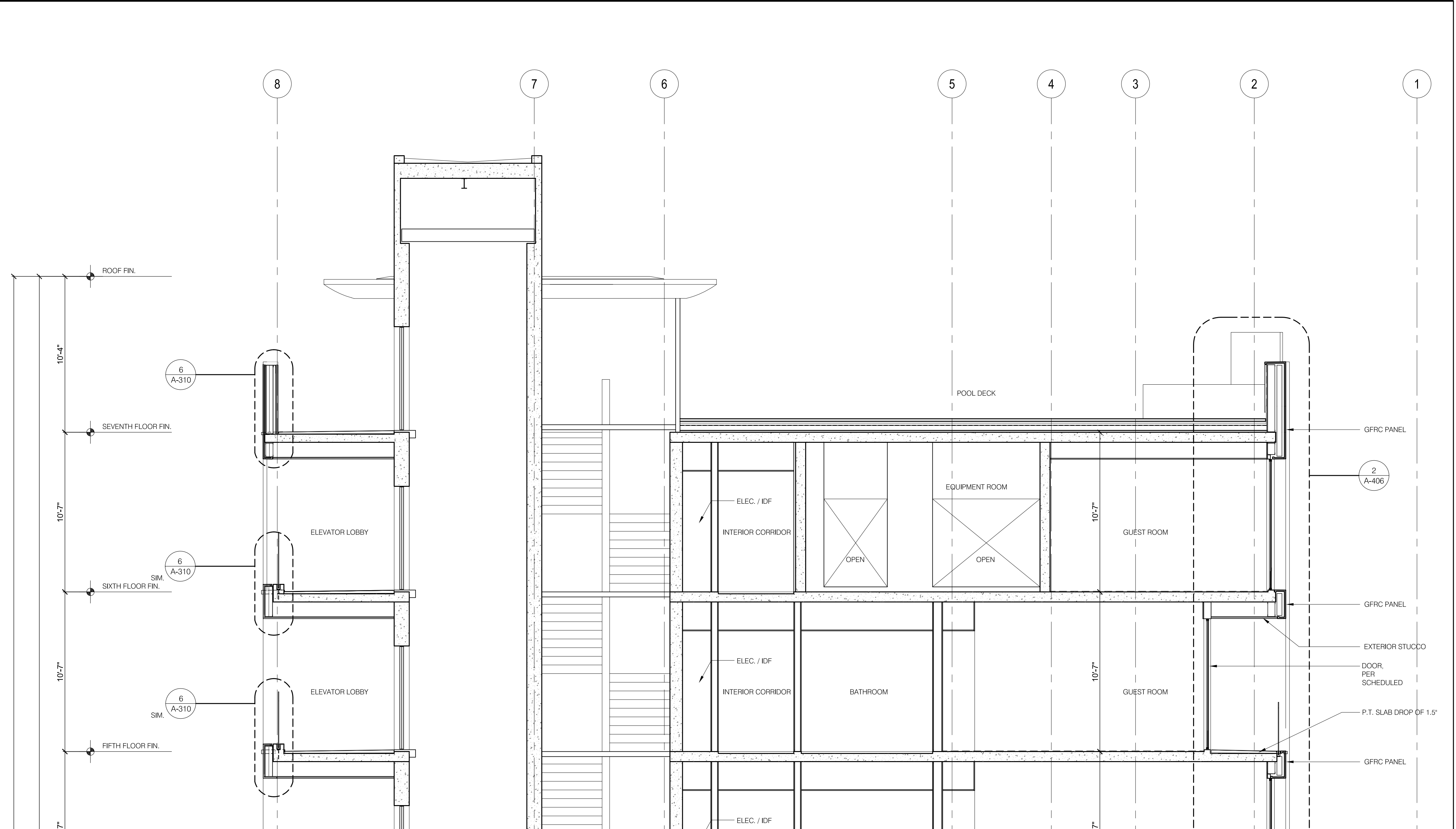
SECTION AT ALLEY REFUSE AREA
