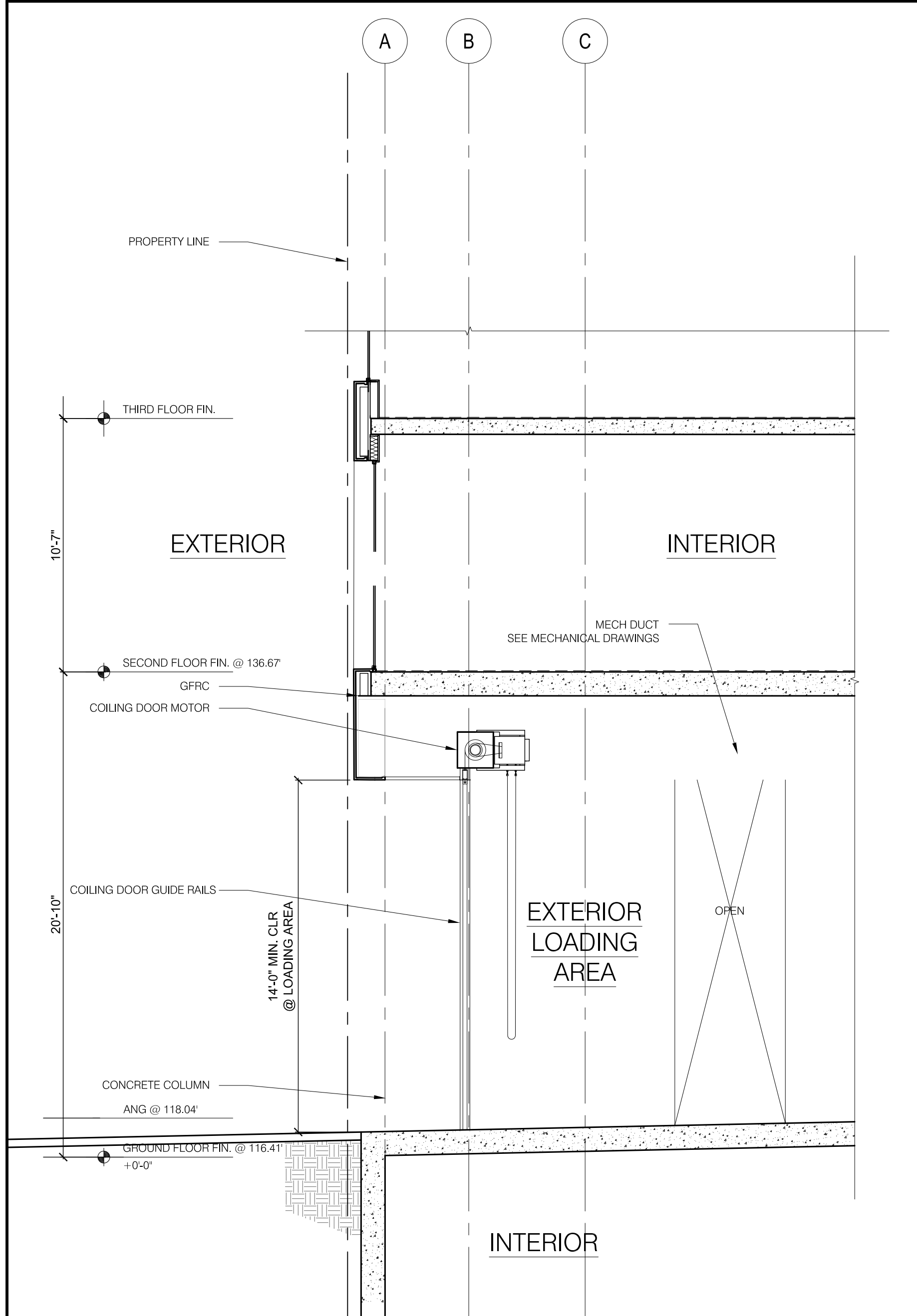
SECTION AT ALLEY LOADING AREA 2 & 3
