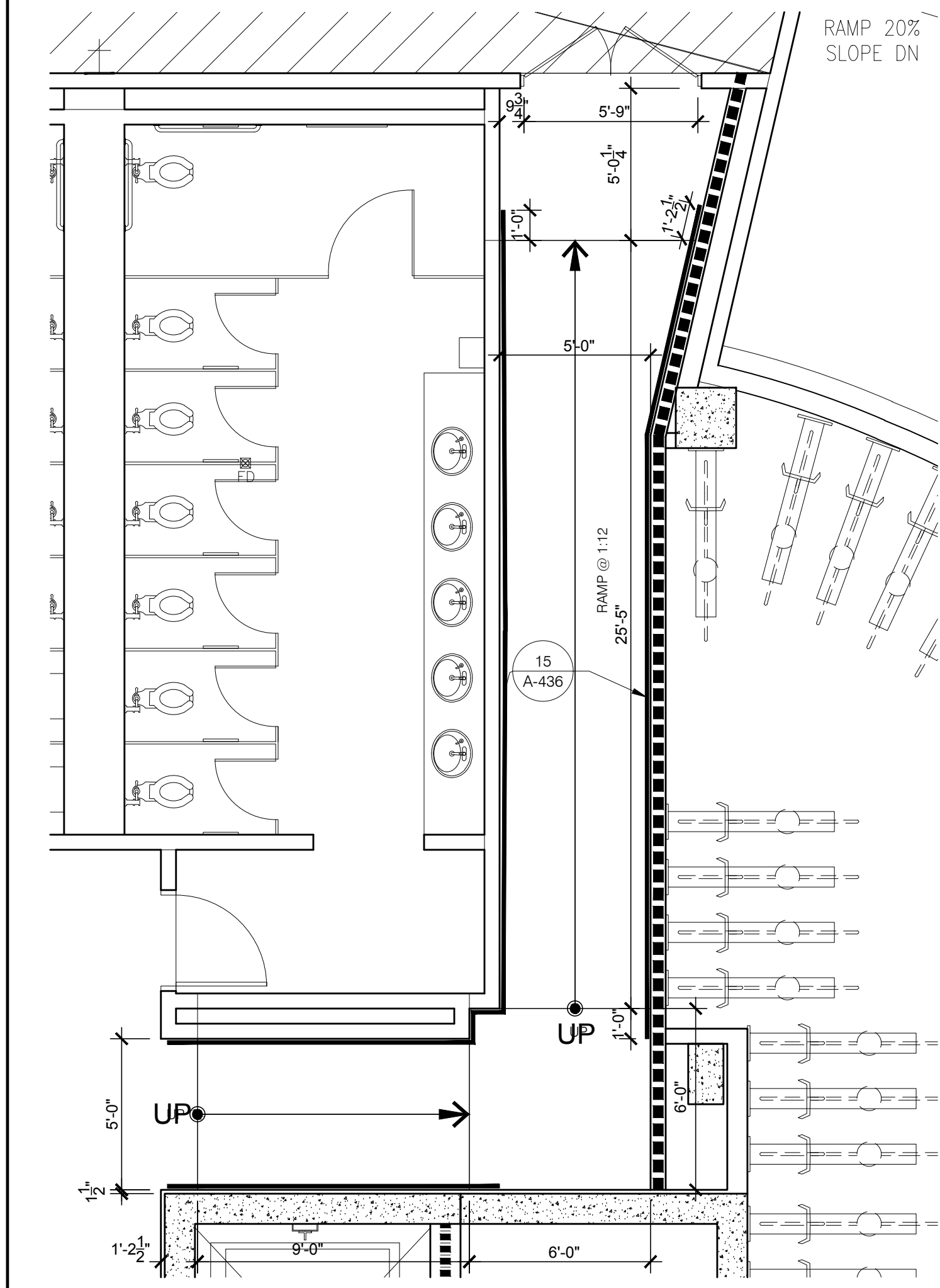
INTERIOR RAMP (IS-3), GROUND
