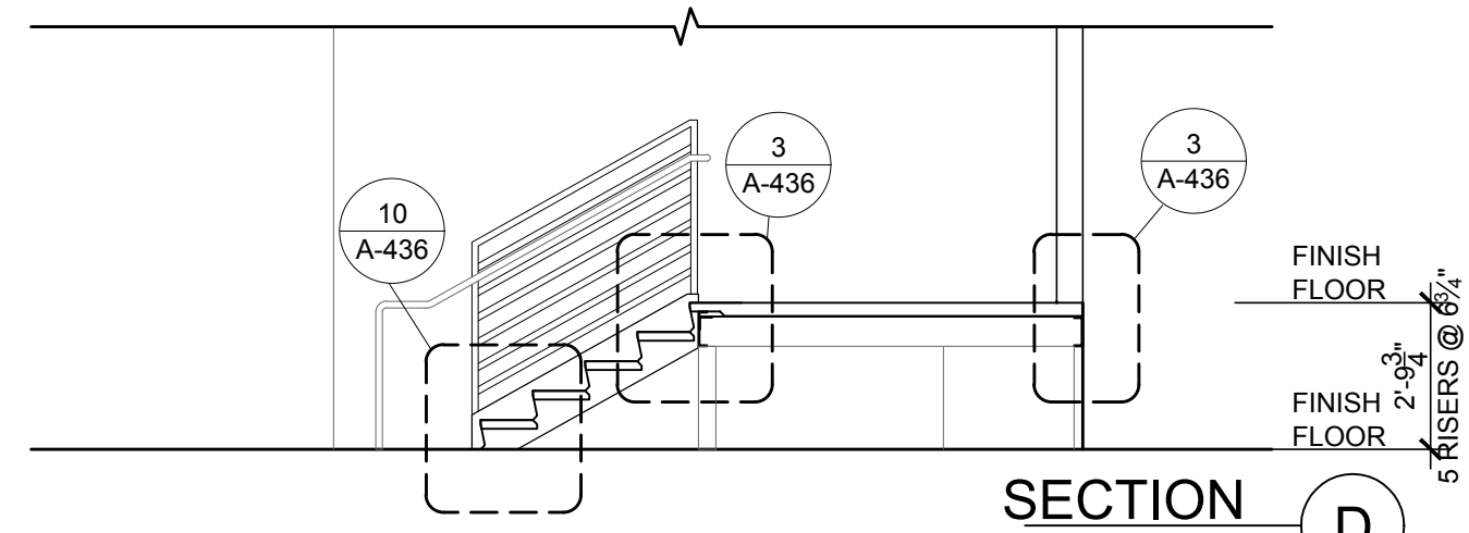
SECTION D
