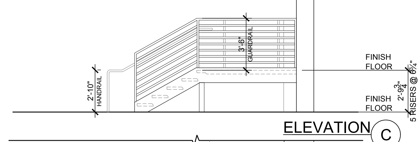
ELEVATION C
