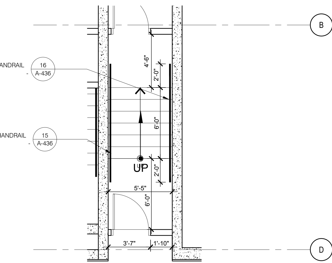
EXTERIOR STAIR (ES-2), GROUND
