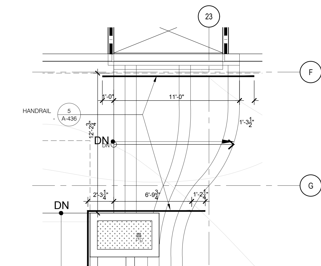
EXTERIOR STAIR (ES-1), GROUND
