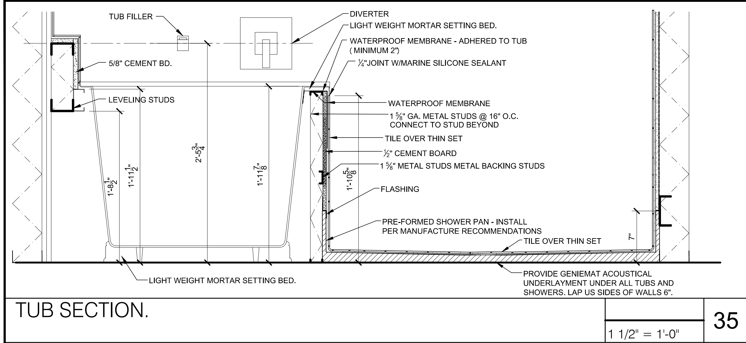
TUB SECTION. 1 1/2" = 1'-0" 35
