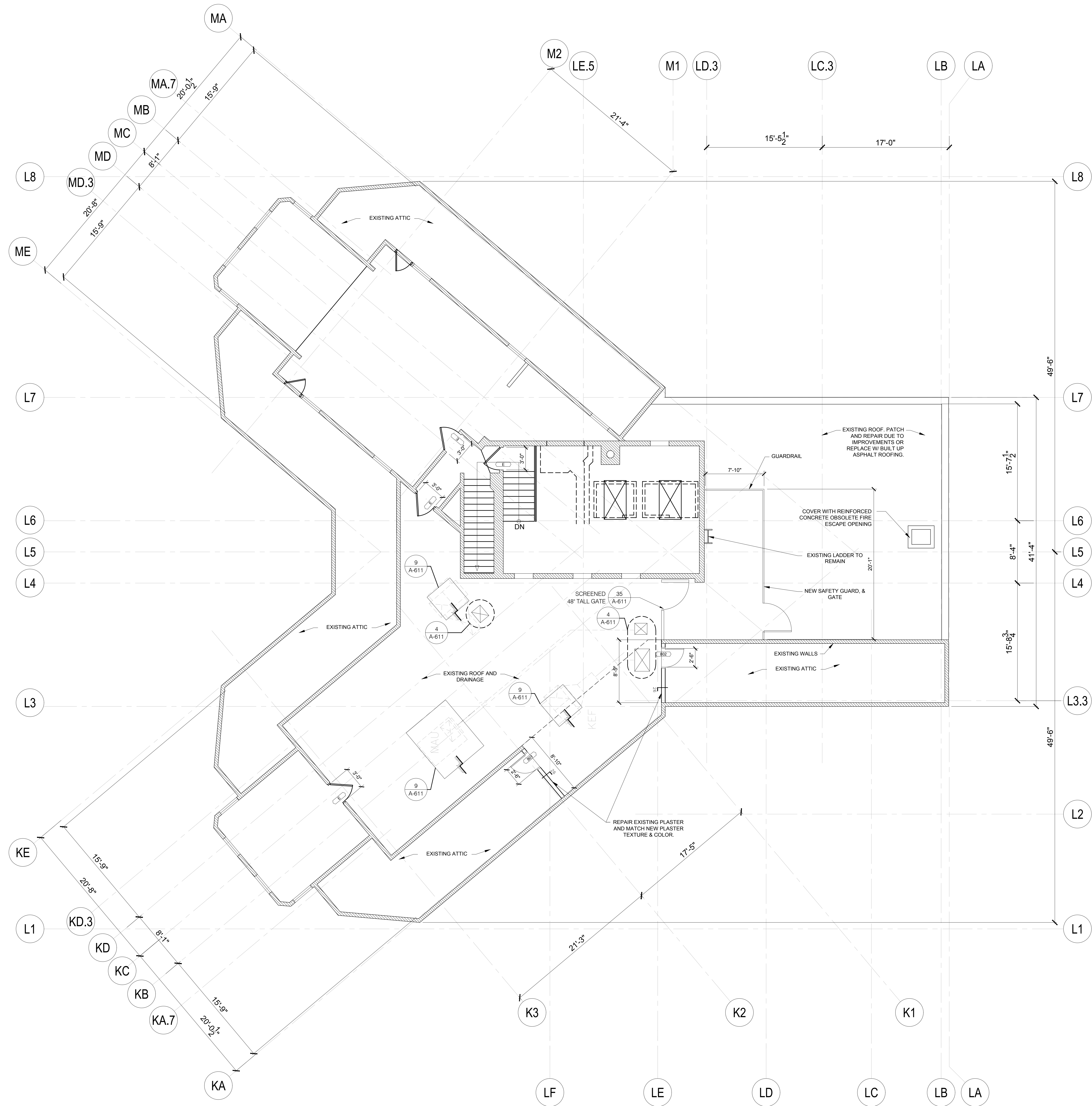
ENLARGED 7TH FLOOR MECHANICAL PLAN - LANDMARK BUILDING
