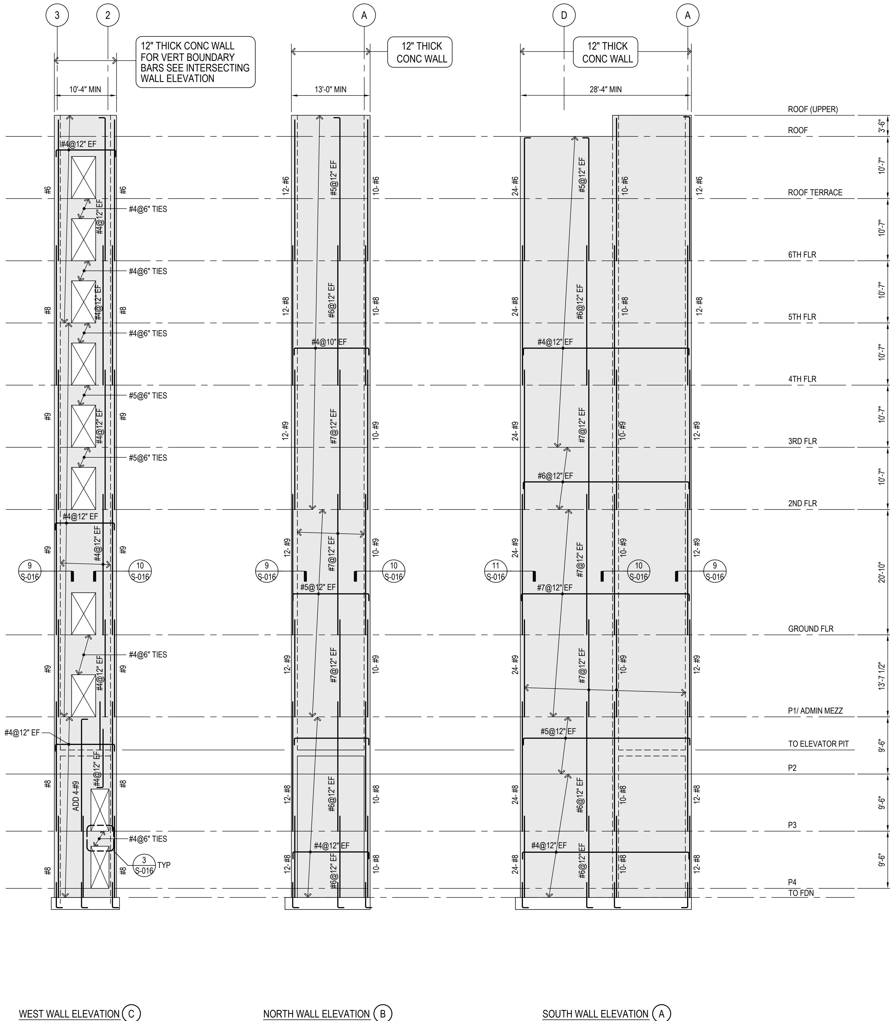
ELEVATOR 5 SHEAR WALL ELEVATIONS
