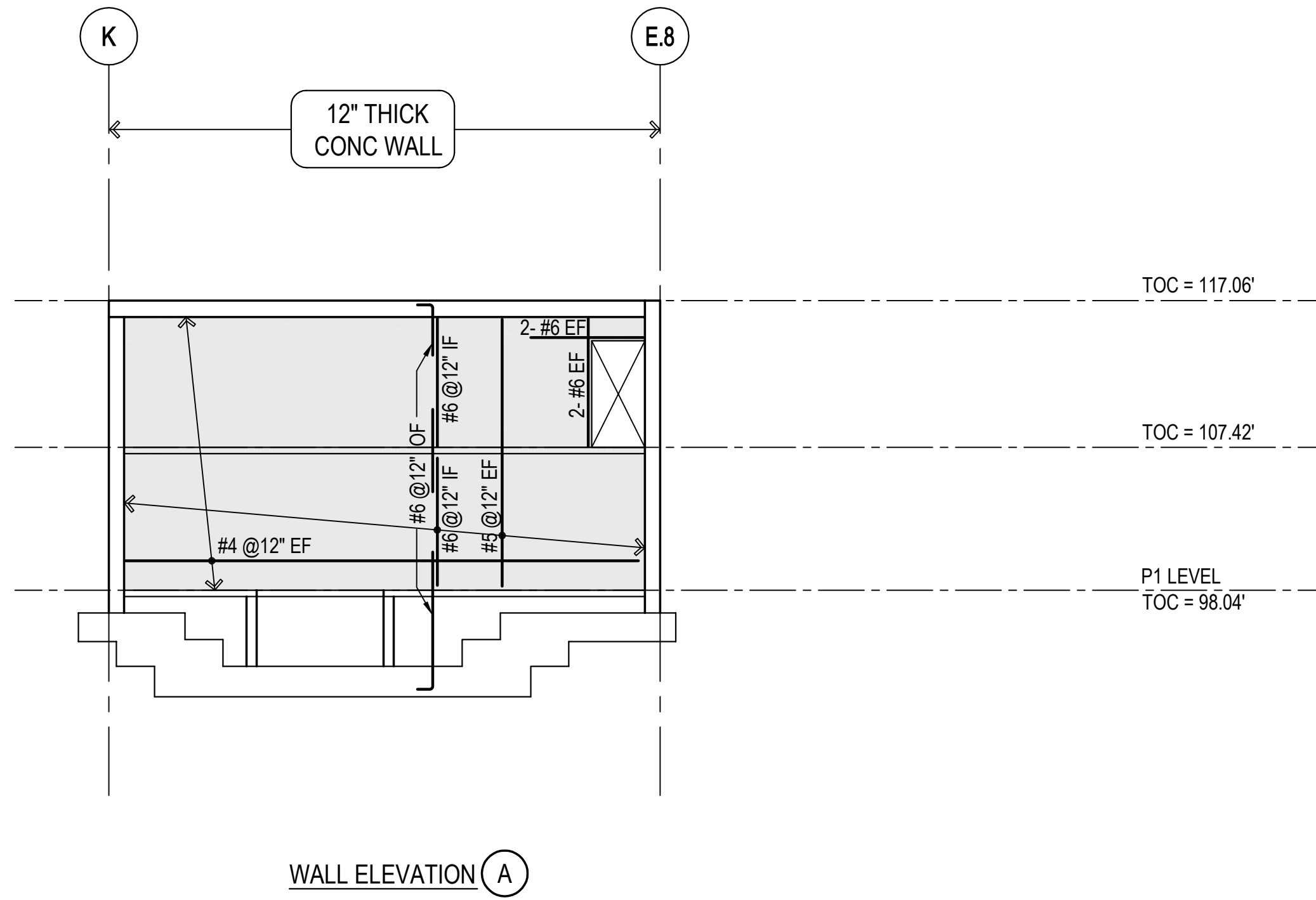
SHEAR WALL ELEVATION ON LINE 23.4
