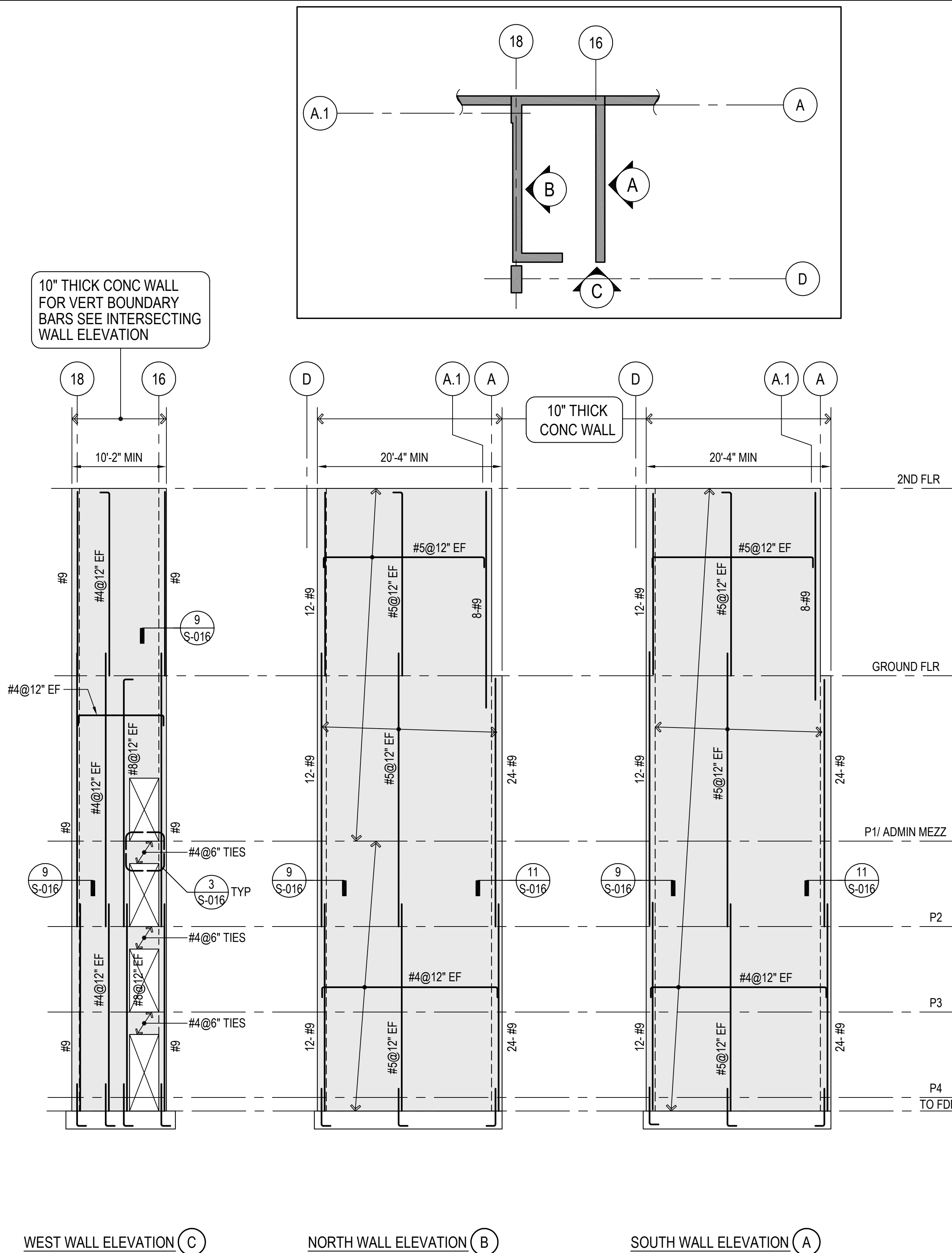
STAIR 5 SHEAR WALL ELEVATIONS
