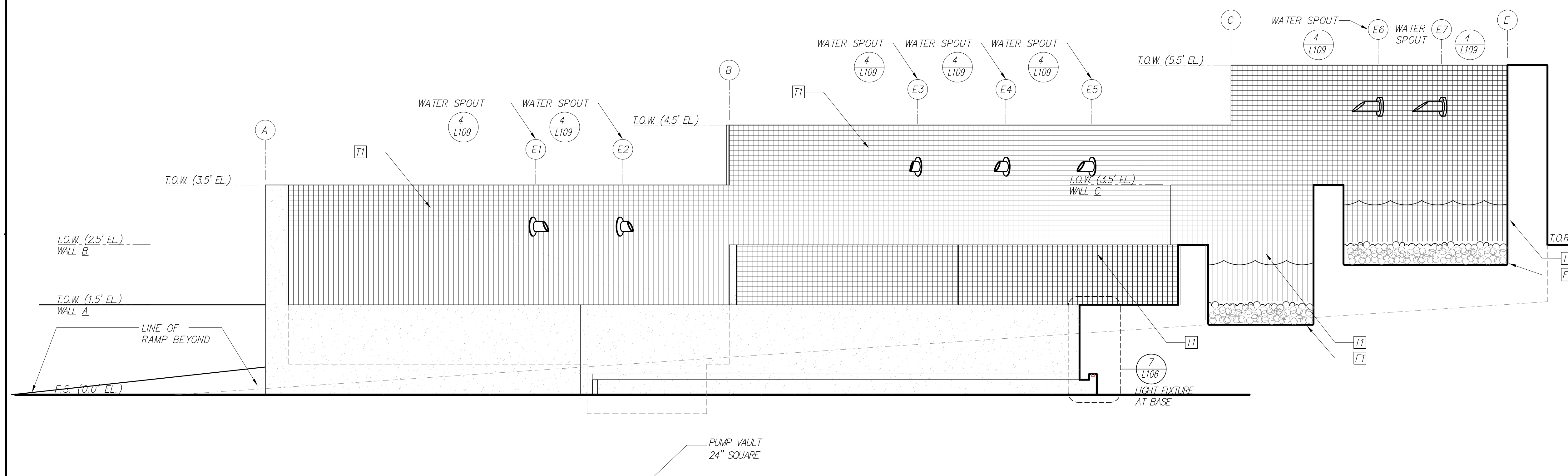
6 PASEO PLANTER AND FOUNTAIN ELEVATION/SECTION
