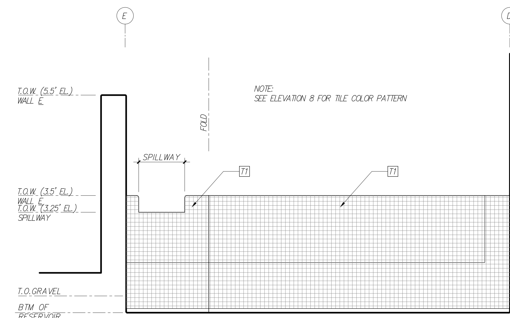
4 FOUNTAIN ELEVATION (SECTION AT LINE D-D) SC: 1" = 1'-0"
