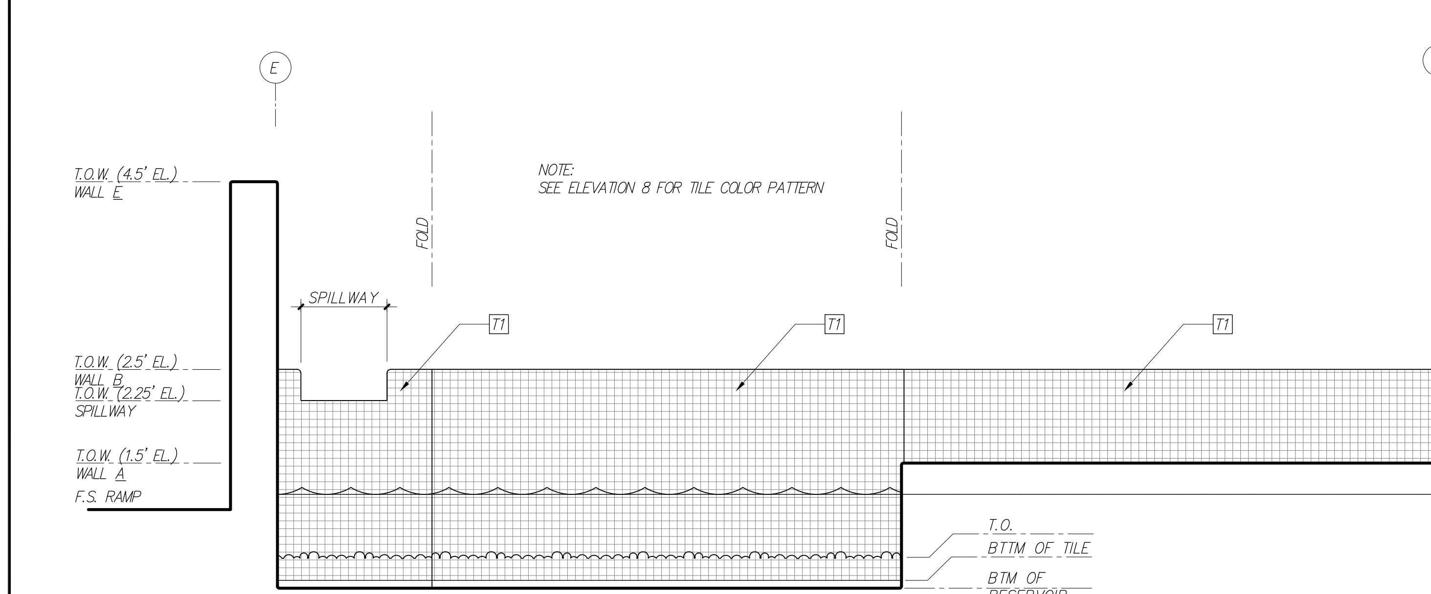
5 FOUNTAIN ELEVATION (SECTION AT LINE B-B)
