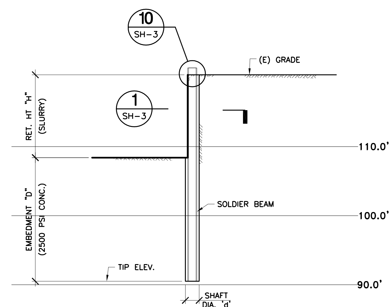
SECTION 1/8" = 1'-0" 10 SH-4
