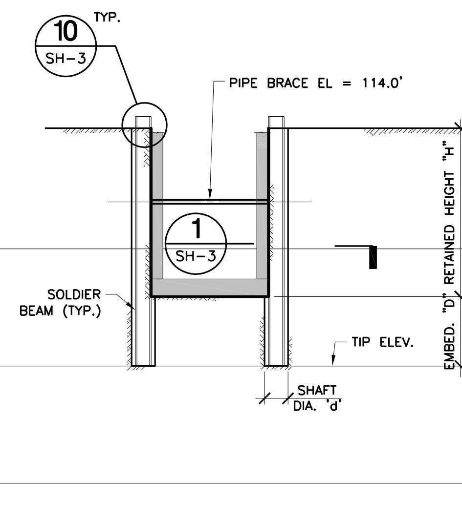
SECTION 1/8" = 1'-0" 9 SH-4
