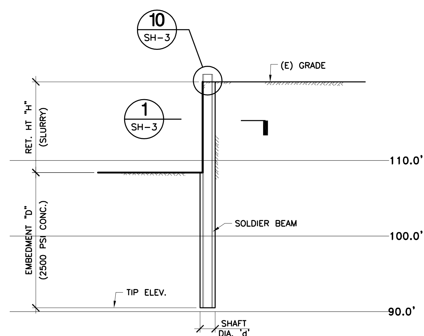
SECTION 1/8" = 1'-0" 10 SH-4
