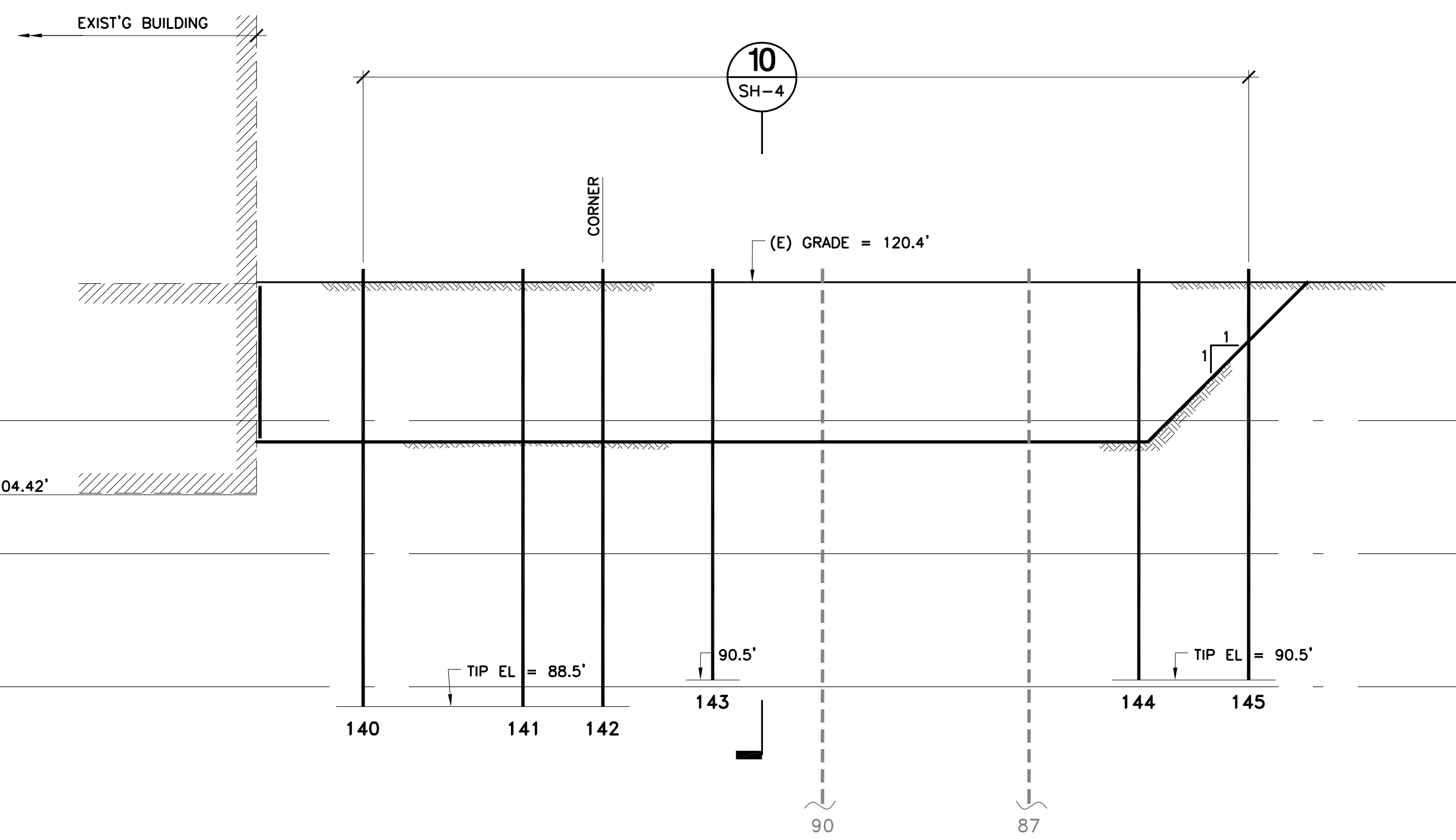
ELEVATION 1/8" = 1'-0" G SH-4
