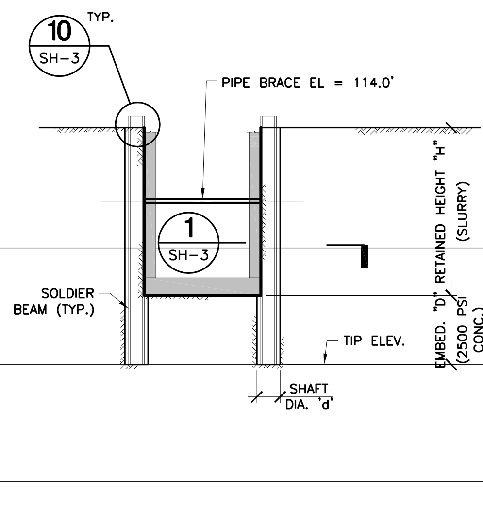
SECTION 1/8" = 1'-0" 9 SH-4
