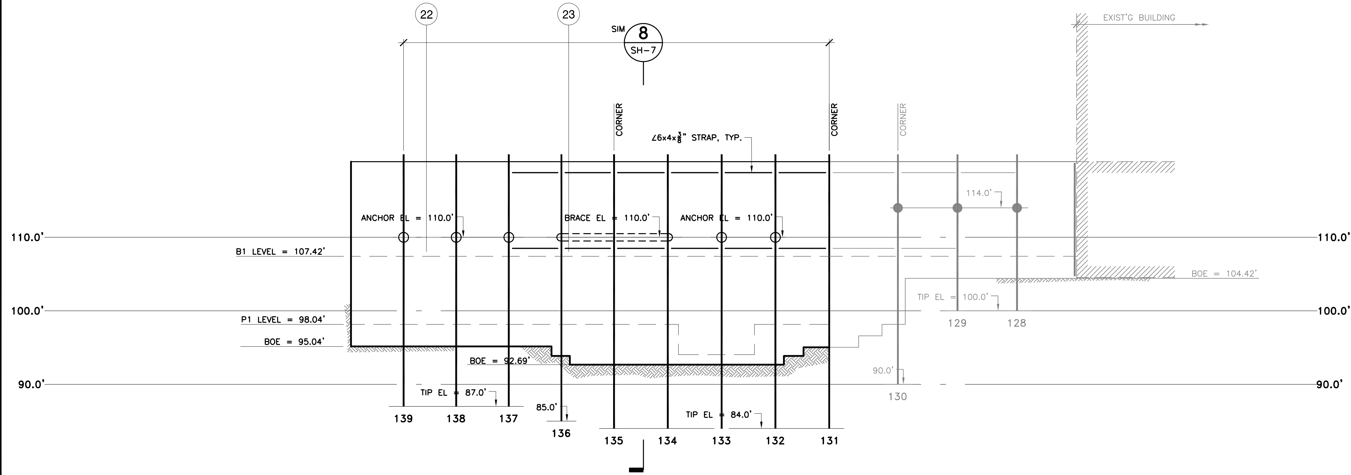
ELEVATION F 1/8" = 1'-0"
