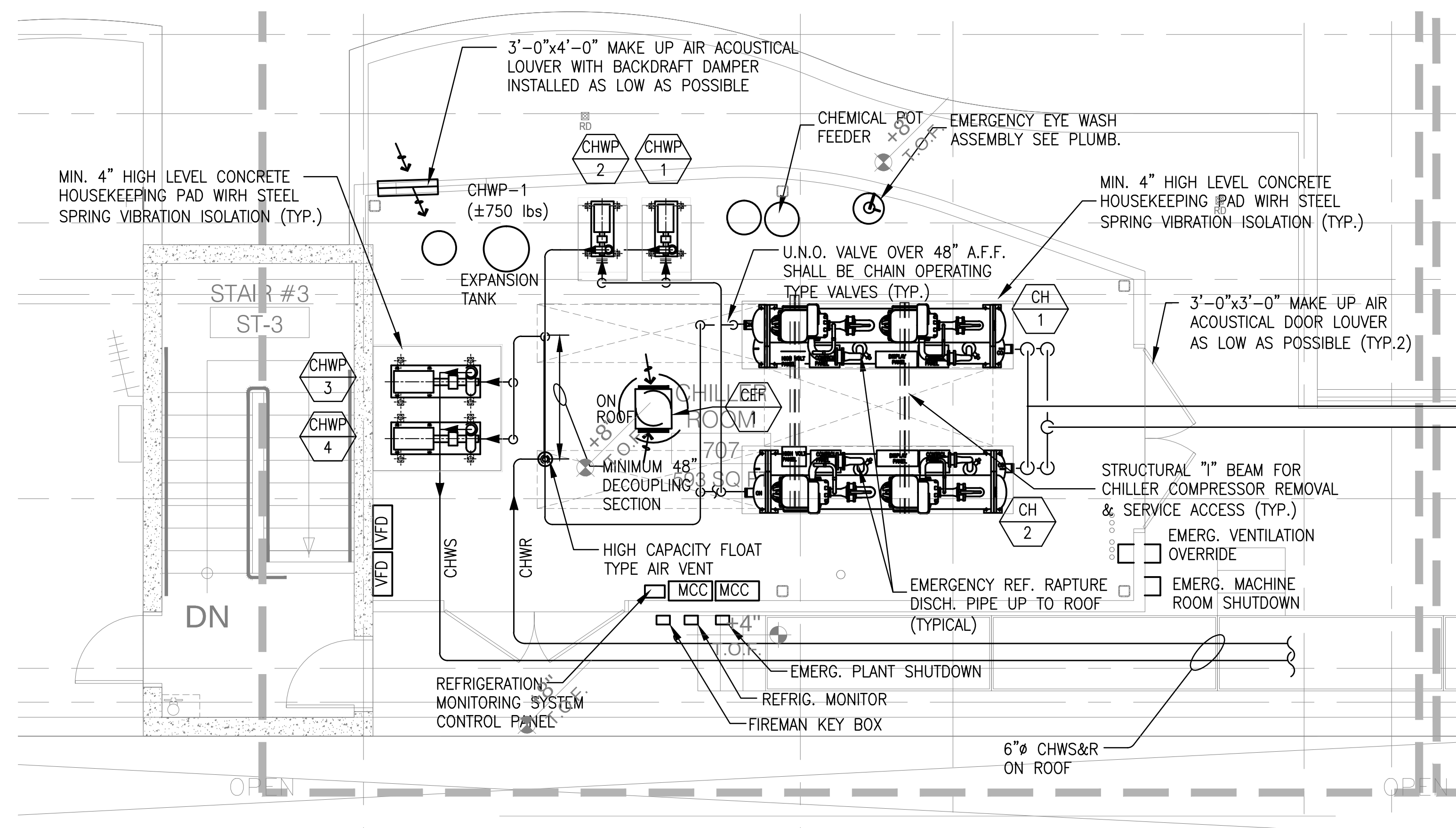
2 ENLARGED SEVENTH FLOOR CHILLER ROOM Scale: 3/8" = 1'-0"
