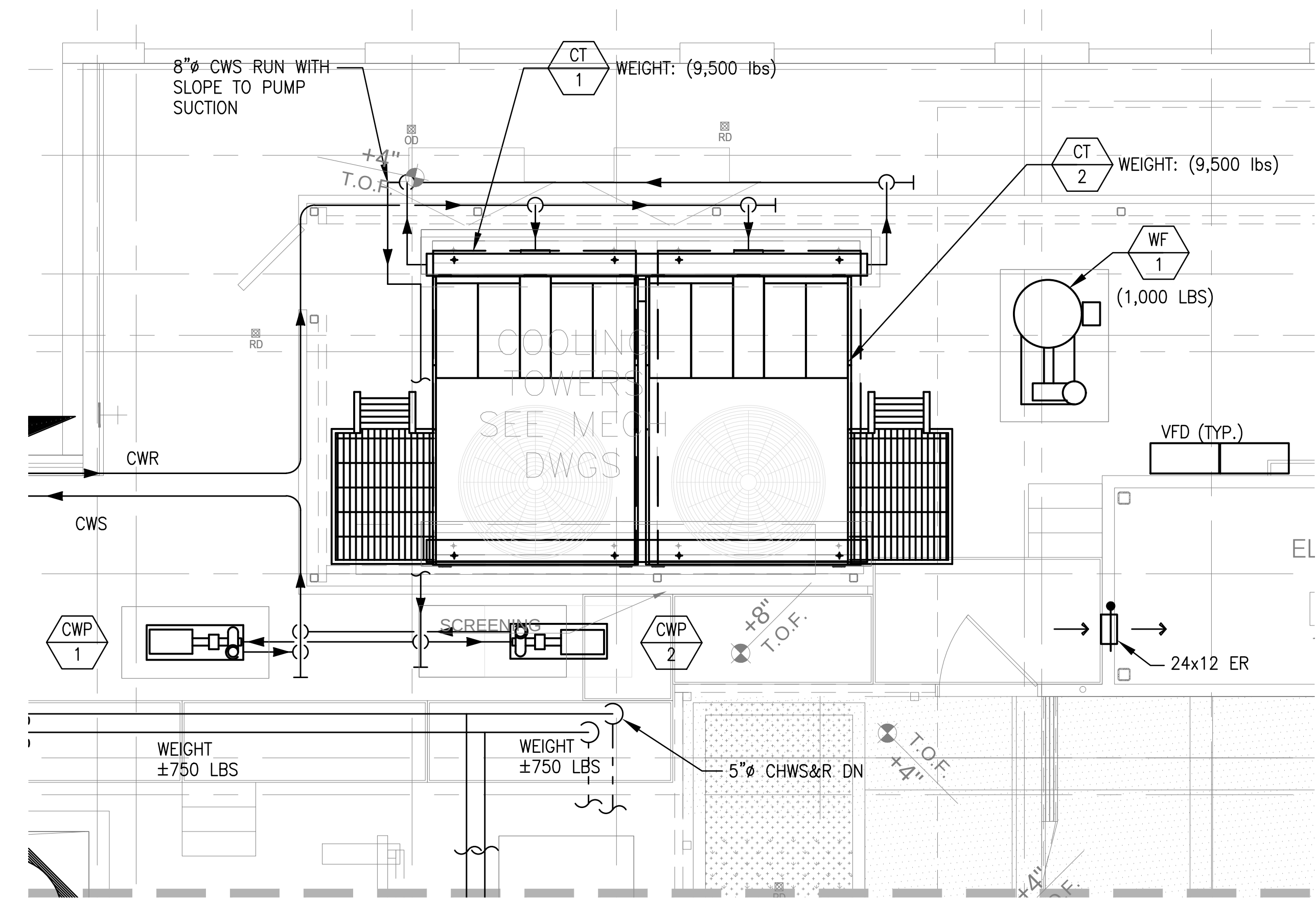
1 ENLARGED SEVENTH FLOOR COOLING TOWER Scale: 3/8" = 1'-0"
