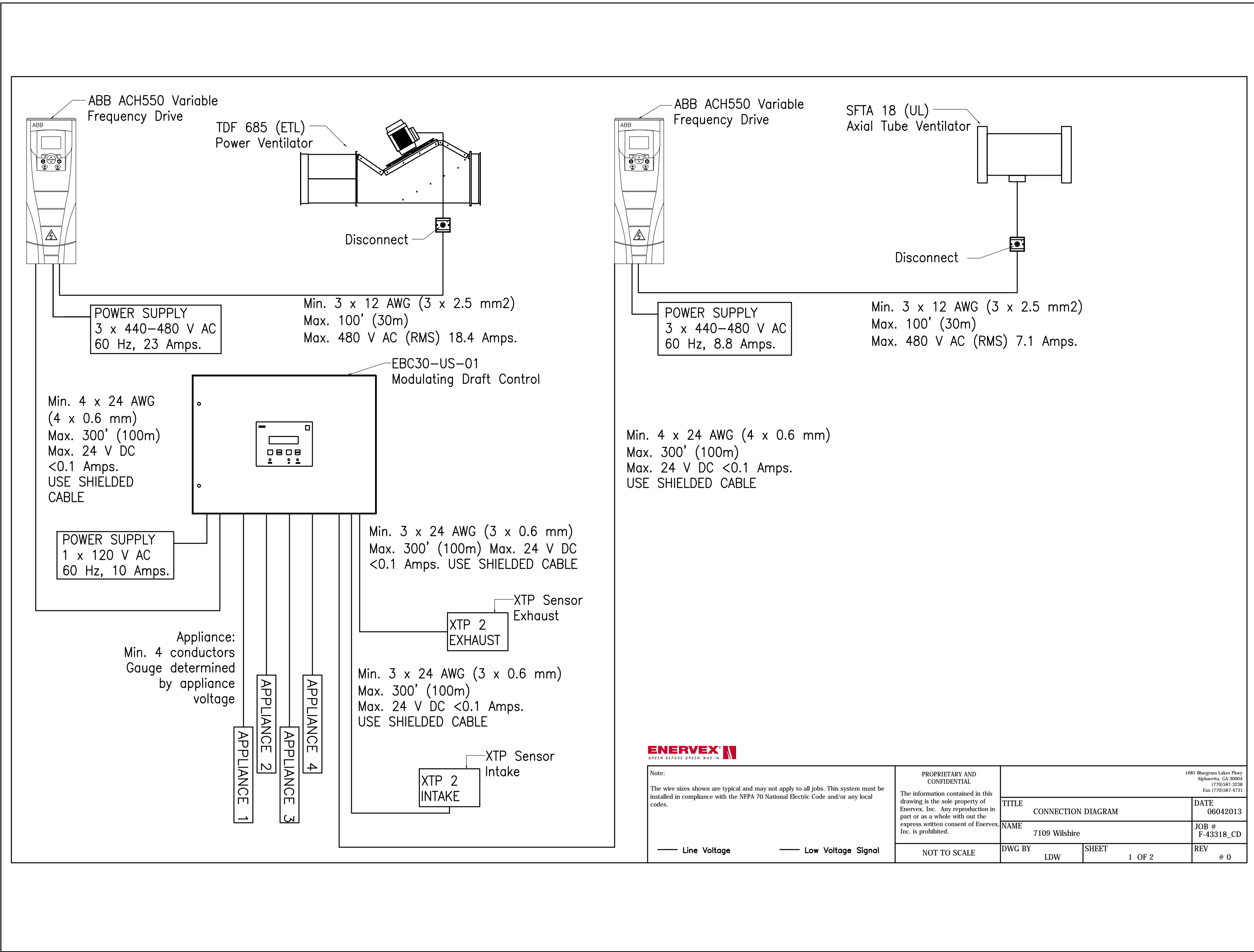
CONNECTION DIAGRAM FOR DRYER EXHAUST FAN AND MAKE UP AIR FAN
