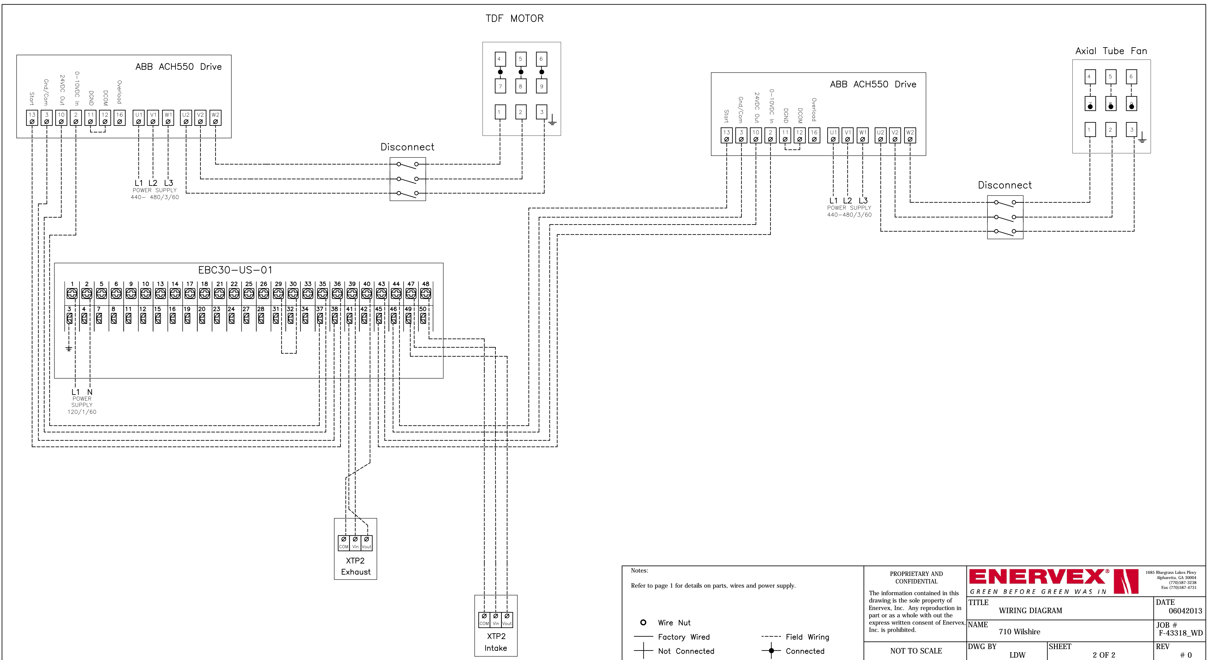
WIRING DIAGRAM
