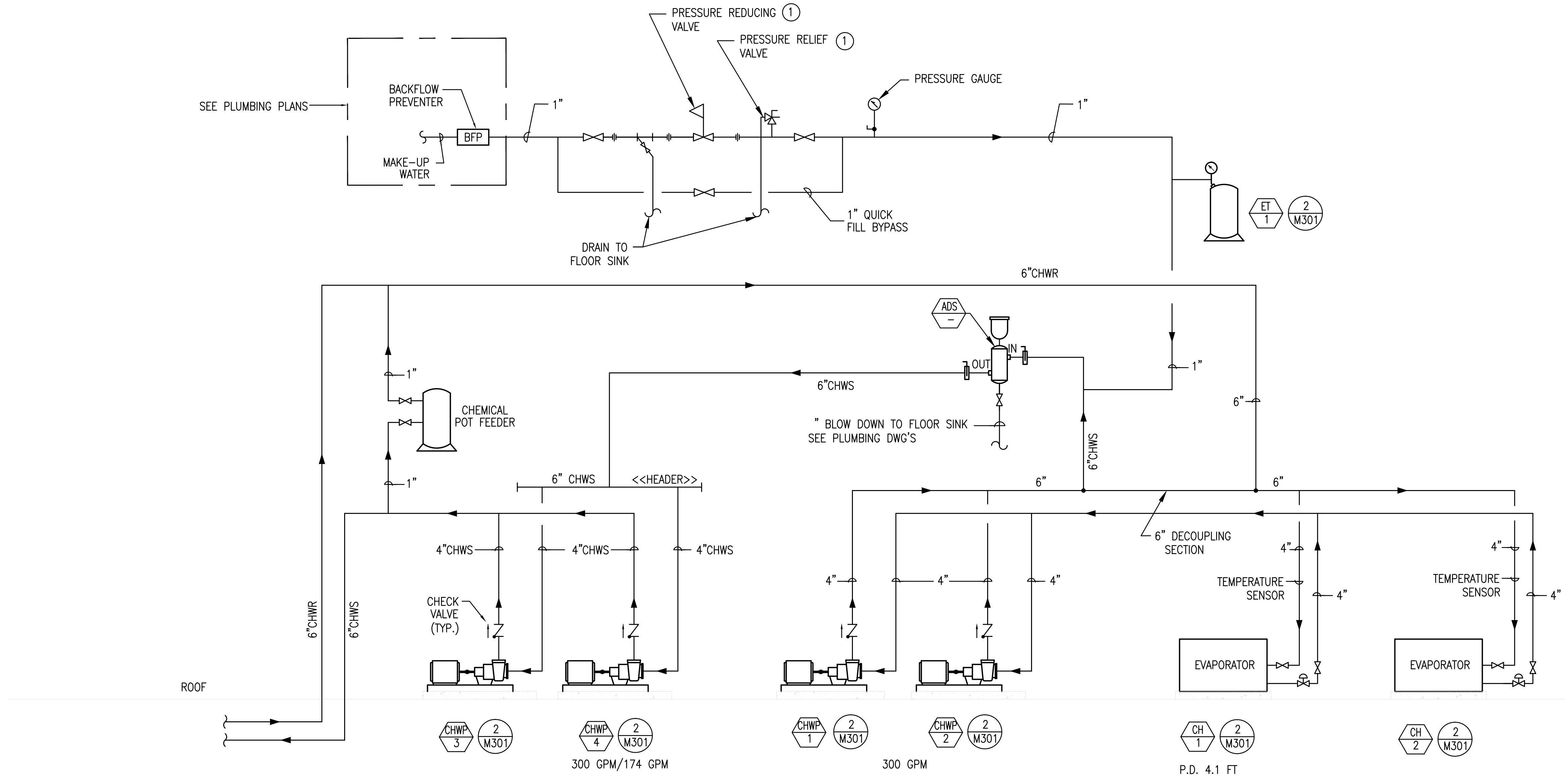
CHILLED WATER PIPING DIAGRAM
