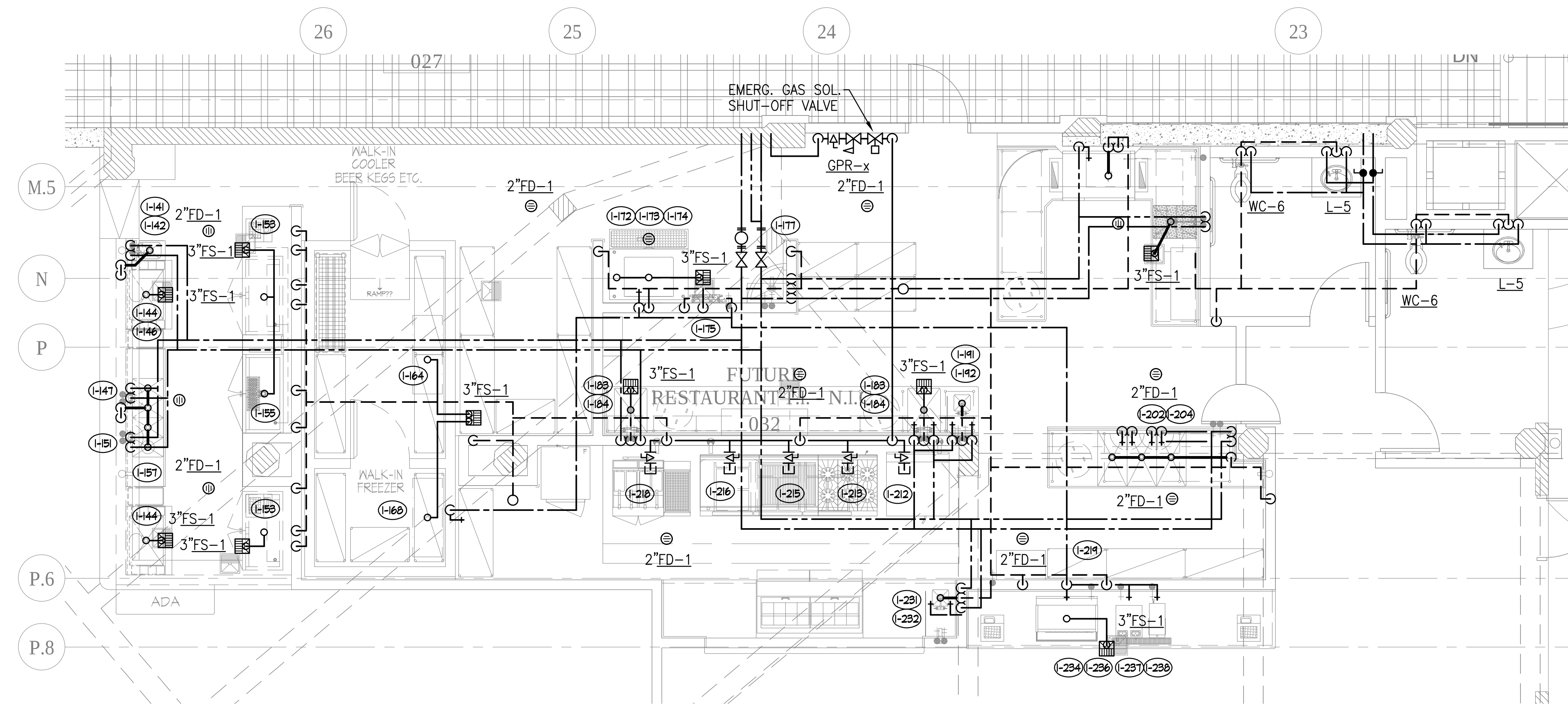
5 ENLARGED GROUND LEVEL LANDMARK RESTAURANT Scale: 1/4" = 1'-0"
