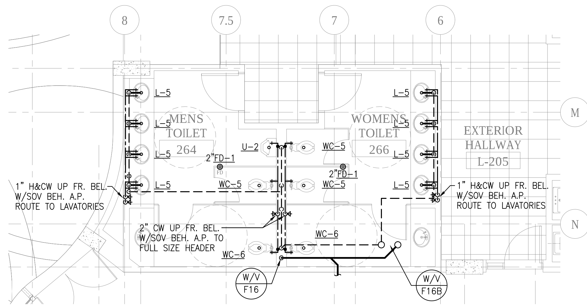
4 ENLARGED LEVEL 2 TOILET ROOM Scale: 1/4" = 1'-0"
