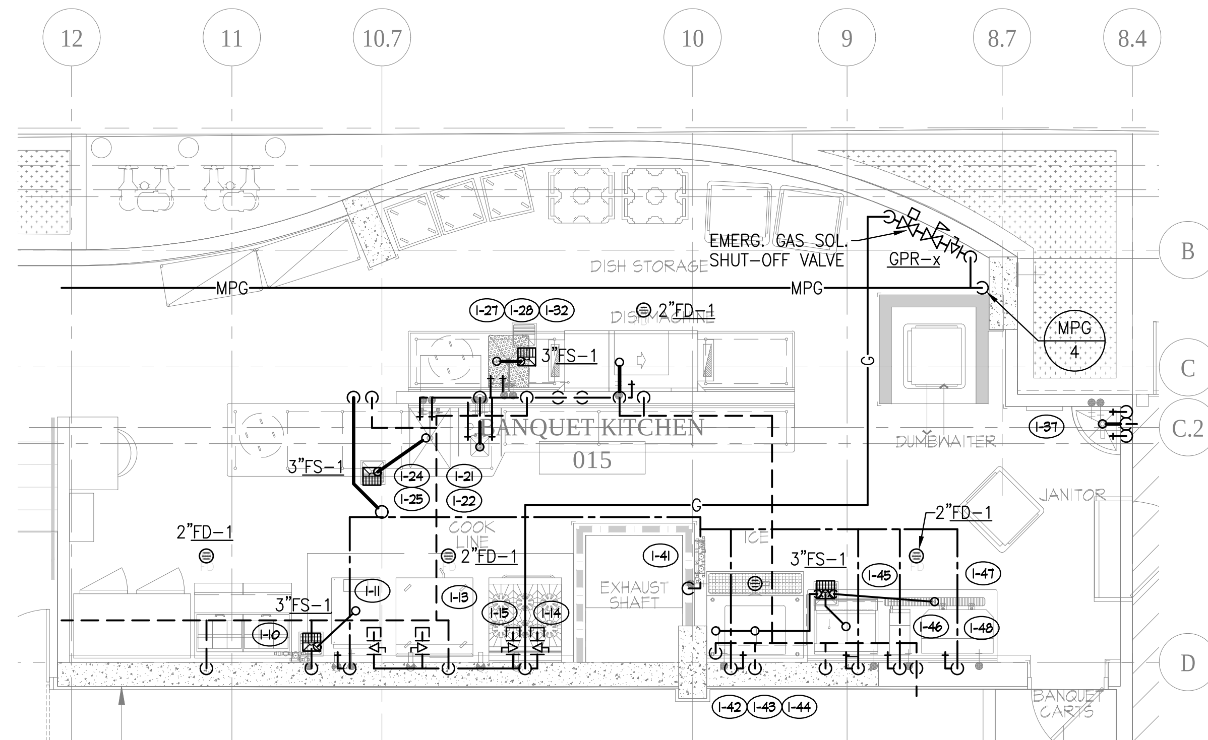
6 ENLARGED GROUND LEVEL BANQUET KITCHEN Scale: 1/4" = 1'-0"
