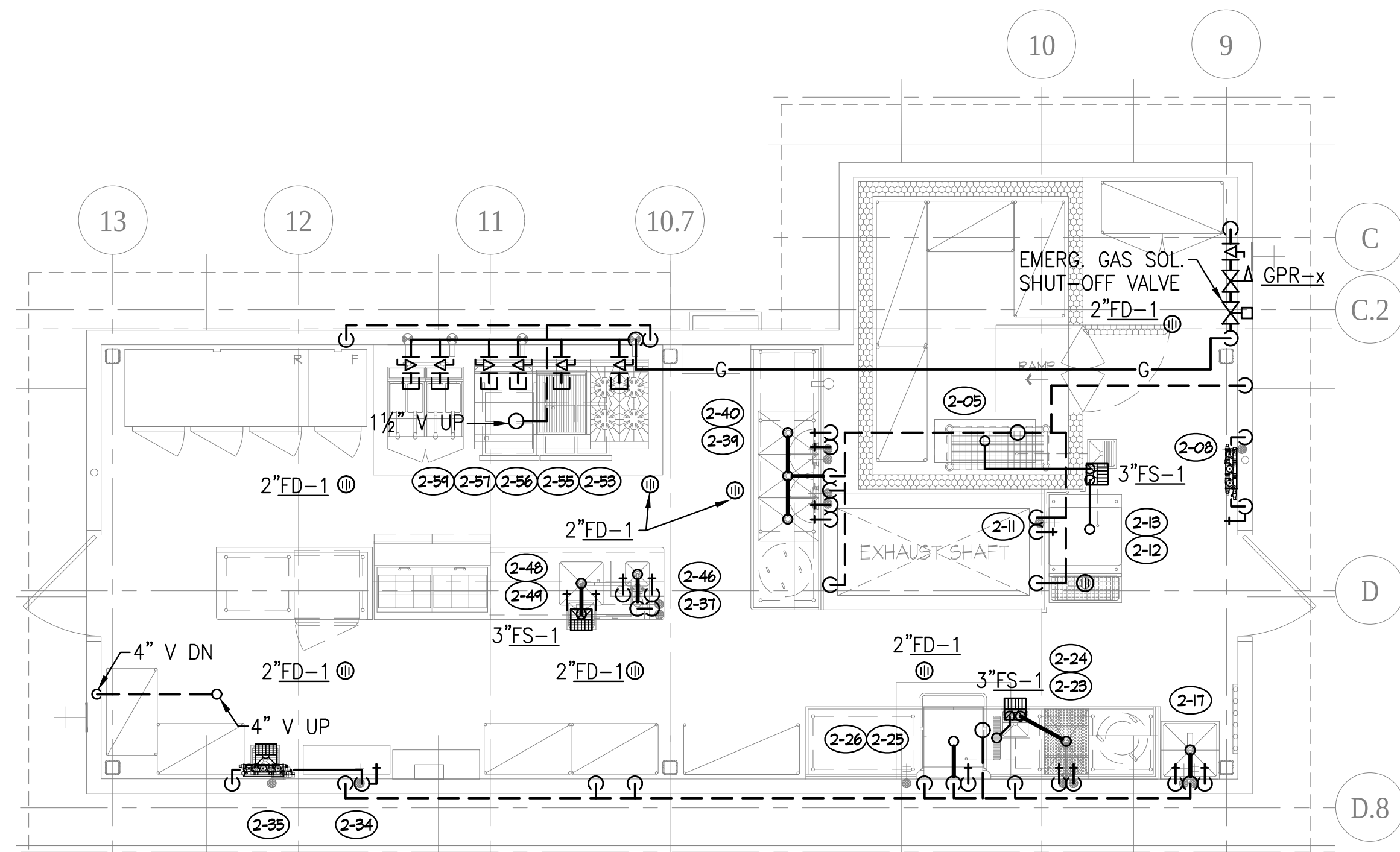
7 ENLARGED LEVEL 7 KITCHEN Scale: 1/4" = 1'-0"
