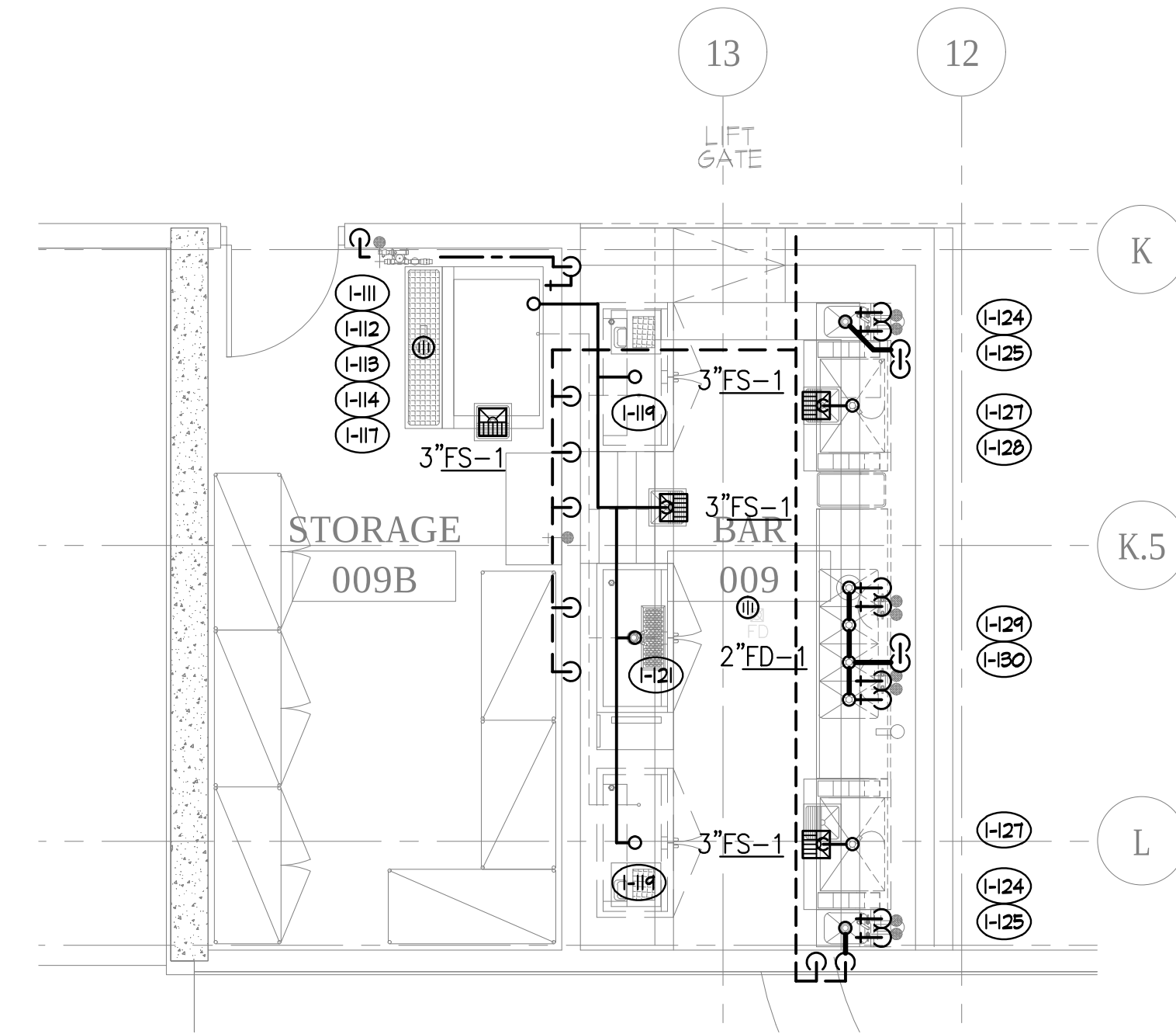
2 ENLARGED GROUND LEVEL PRE-FUNCTION BAR Scale: 1/4" = 1'-0"
