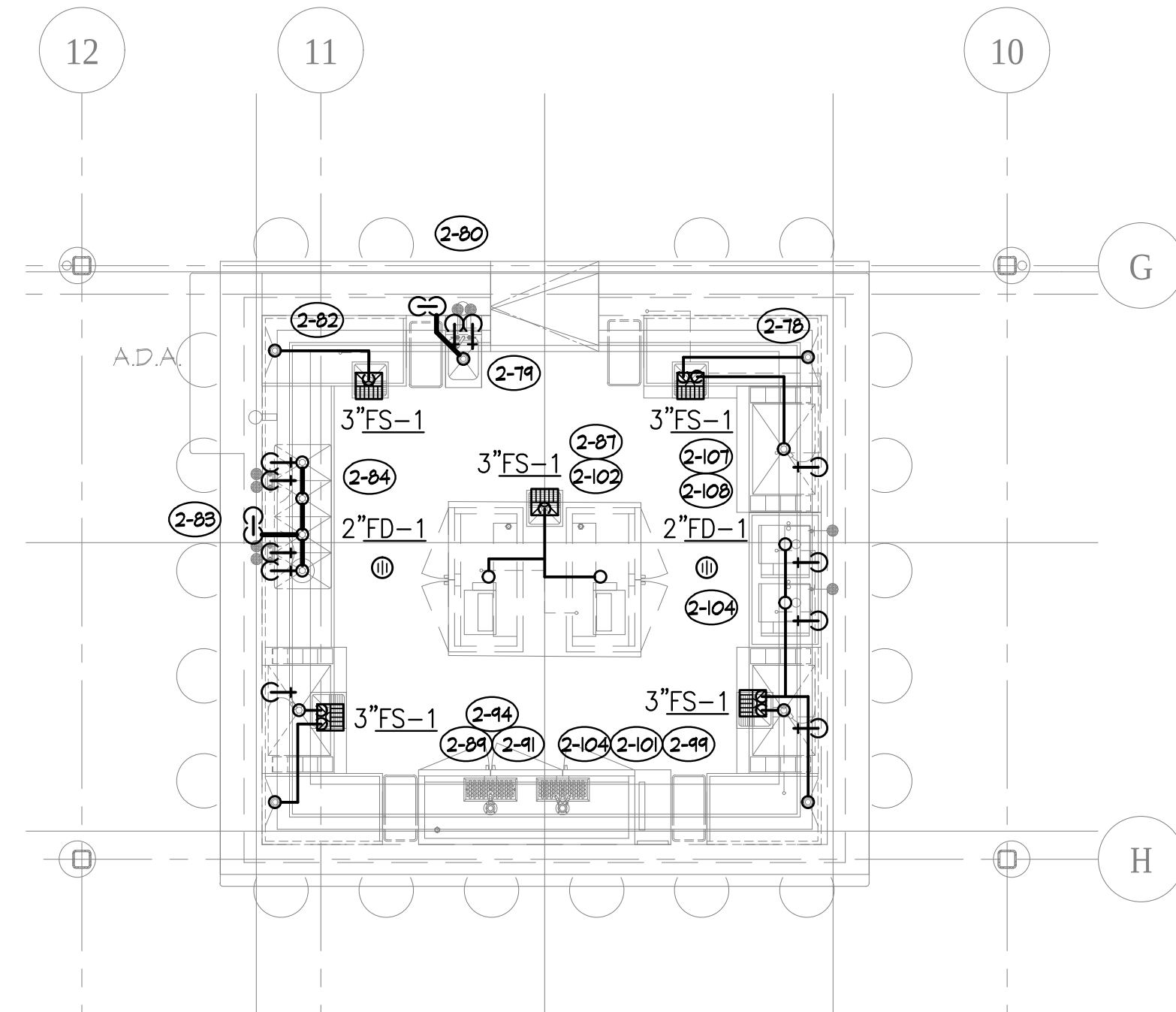
3 ENLARGED LEVEL 7 COCKTAIL BAR Scale: 1/4" = 1'-0"
