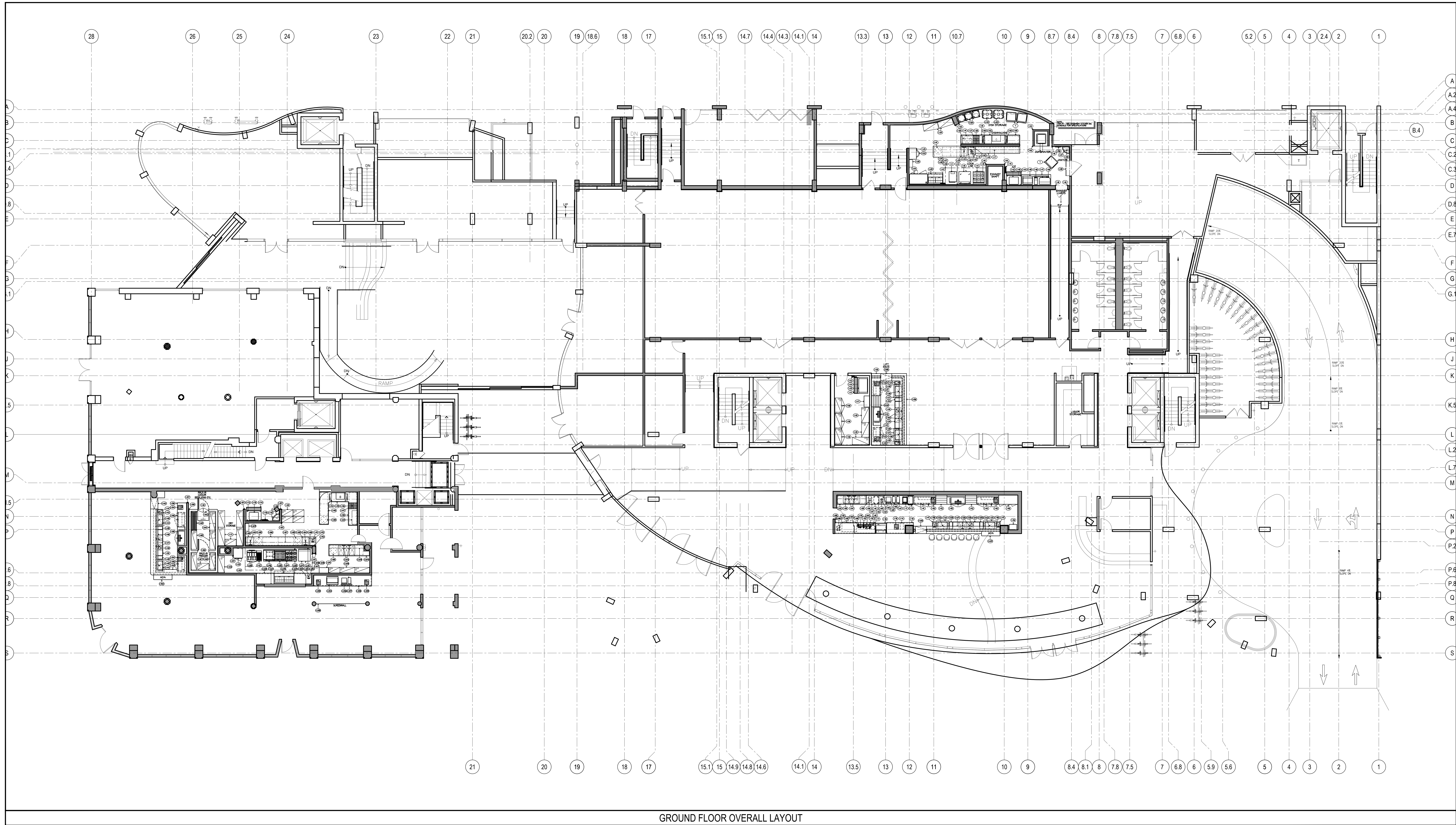
GROUND FLOOR OVERALL LAYOUT
