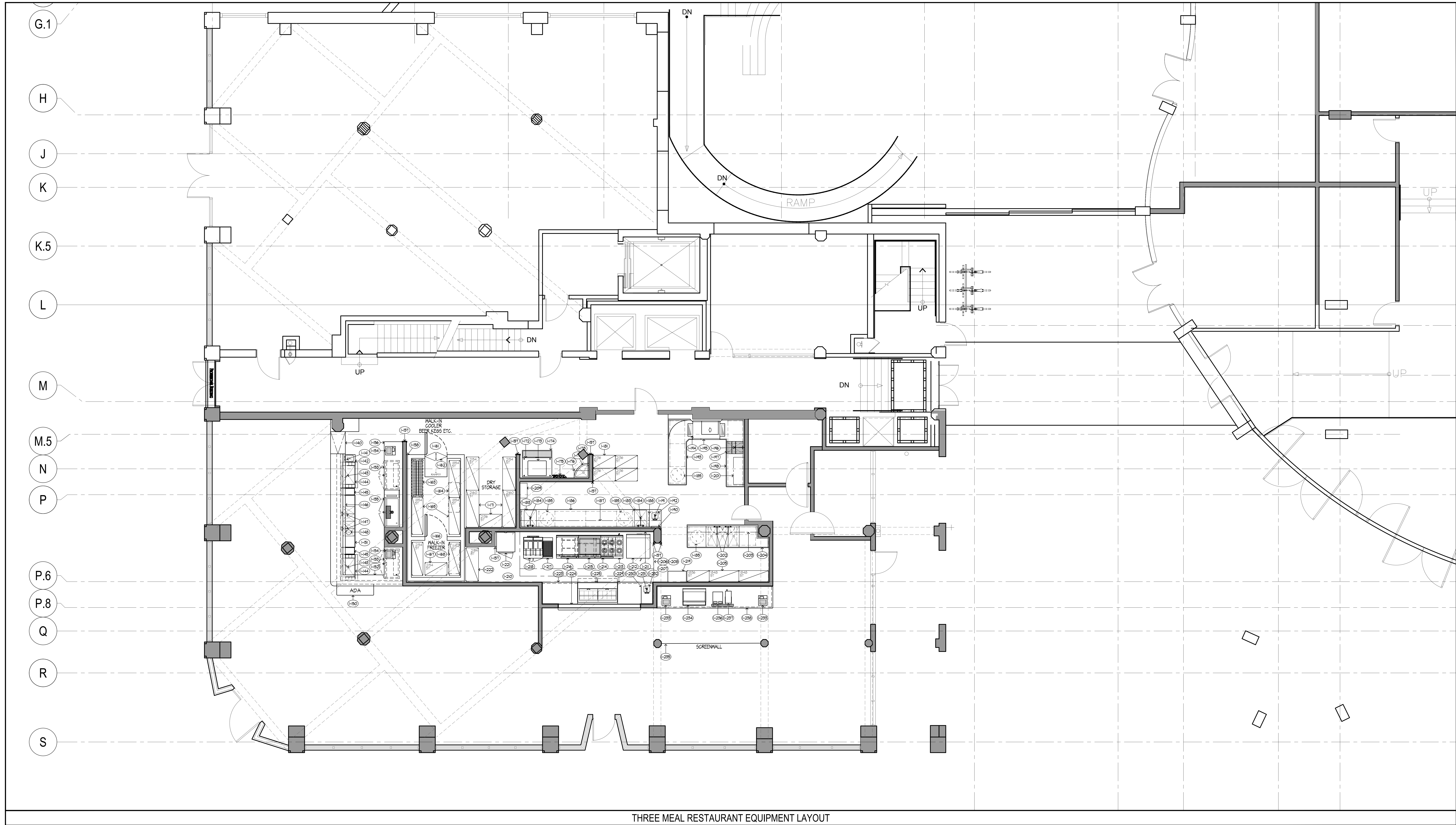
THREE MEAL RESTAURANT EQUIPMENT LAYOUT
