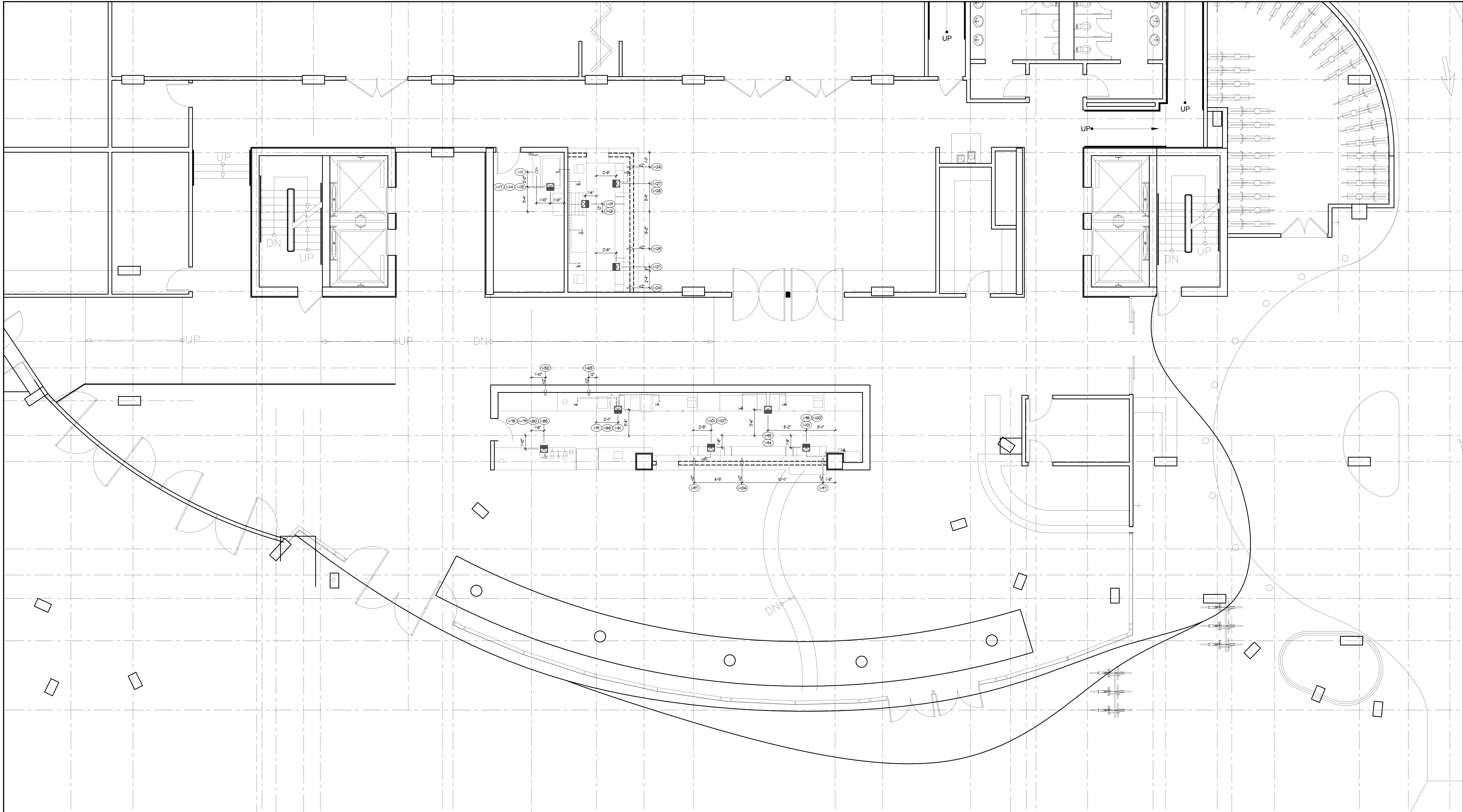
LOBBY BAR FLOOR PENETRATION PLAN
