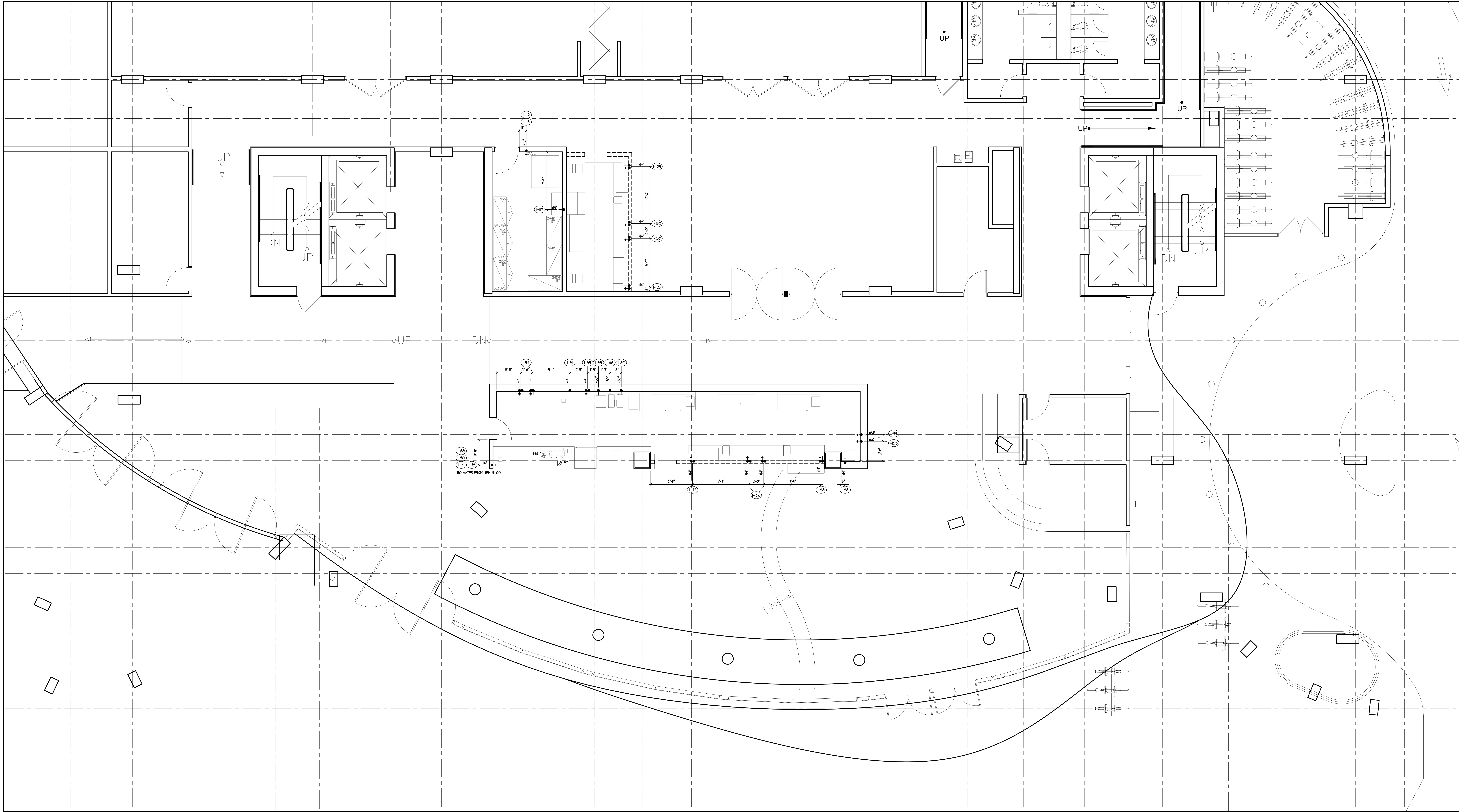
LOBBY BAR PLUMBING PLAN
