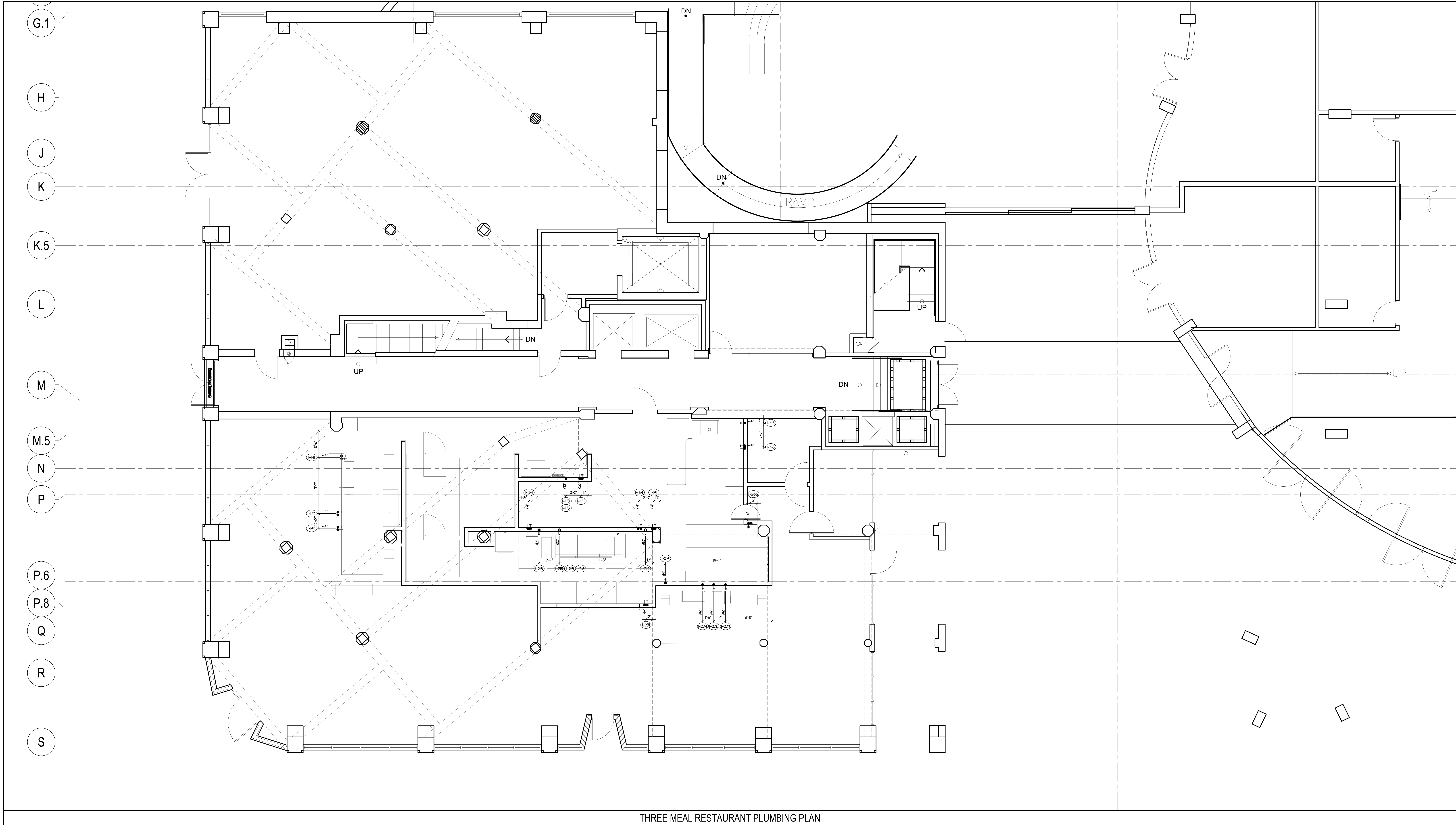
THREE MEAL RESTAURANT PLUMBING PLAN
