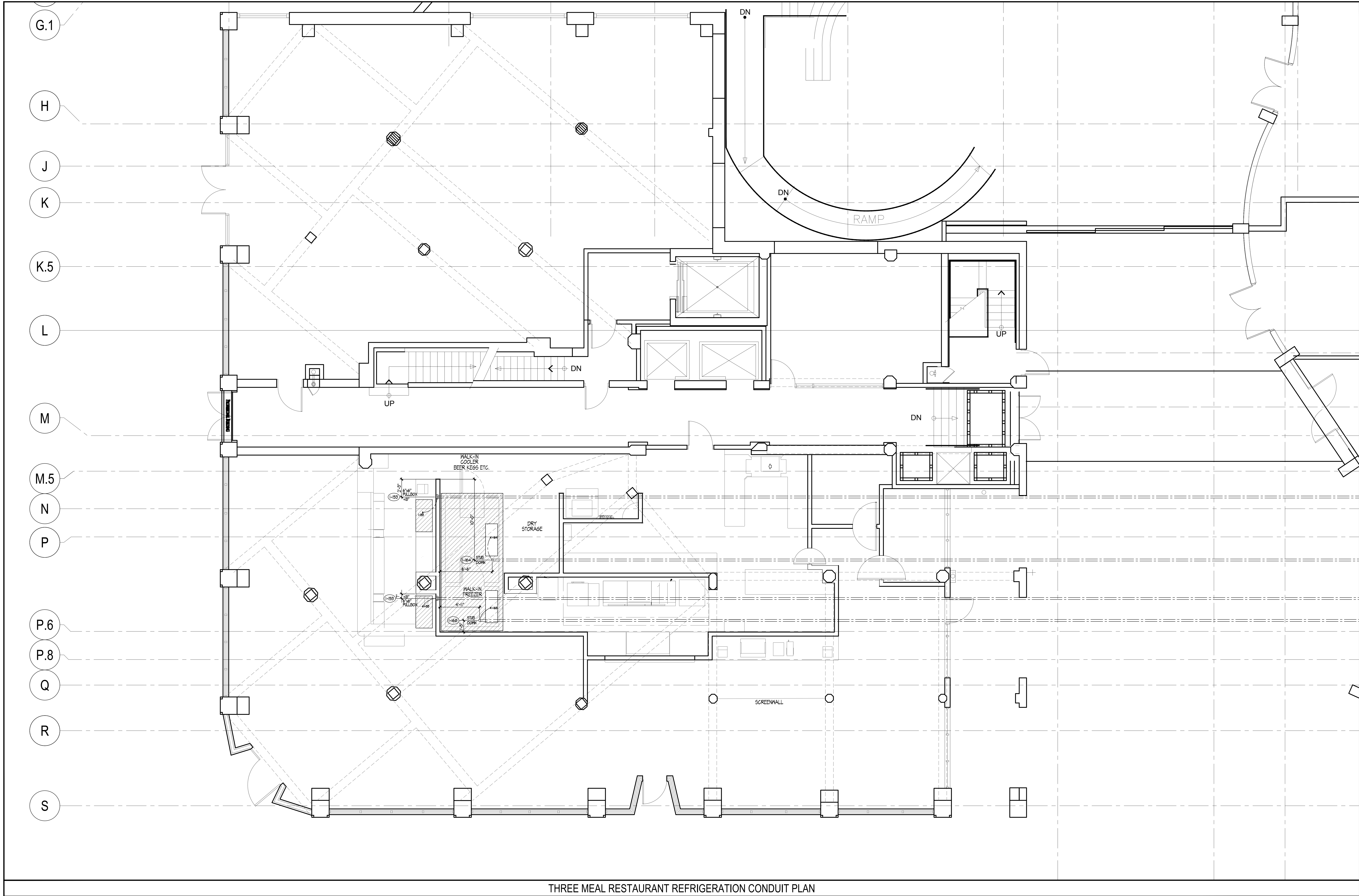
THREE MEAL RESTAURANT REFRIGERATION CONDUIT PLAN
