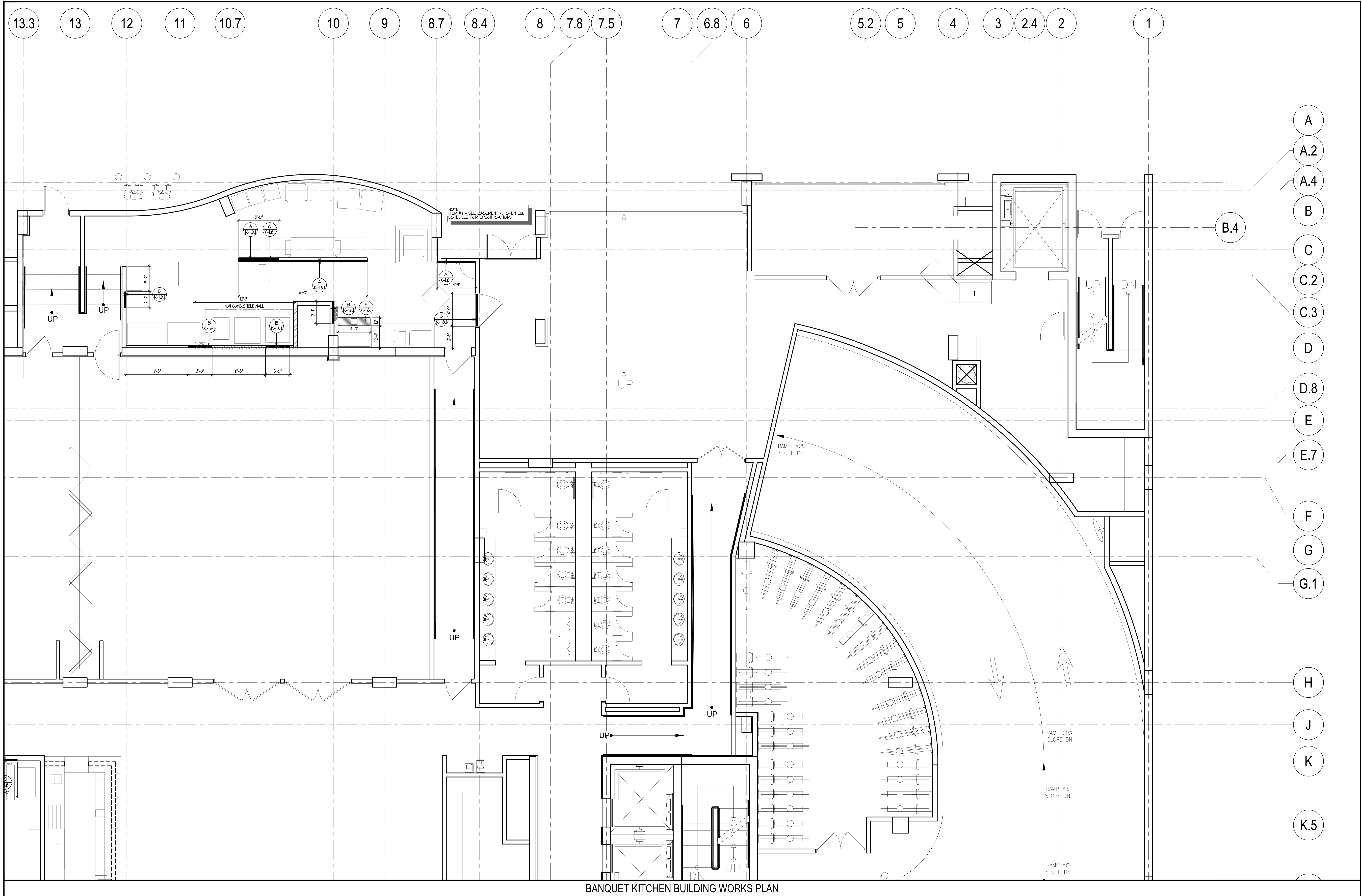
BANQUET KITCHEN BUILDING WORKS PLAN
