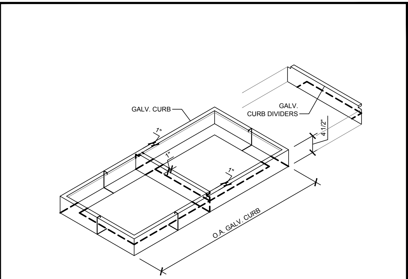
TYP. GALVANIZED CURB PLAN
